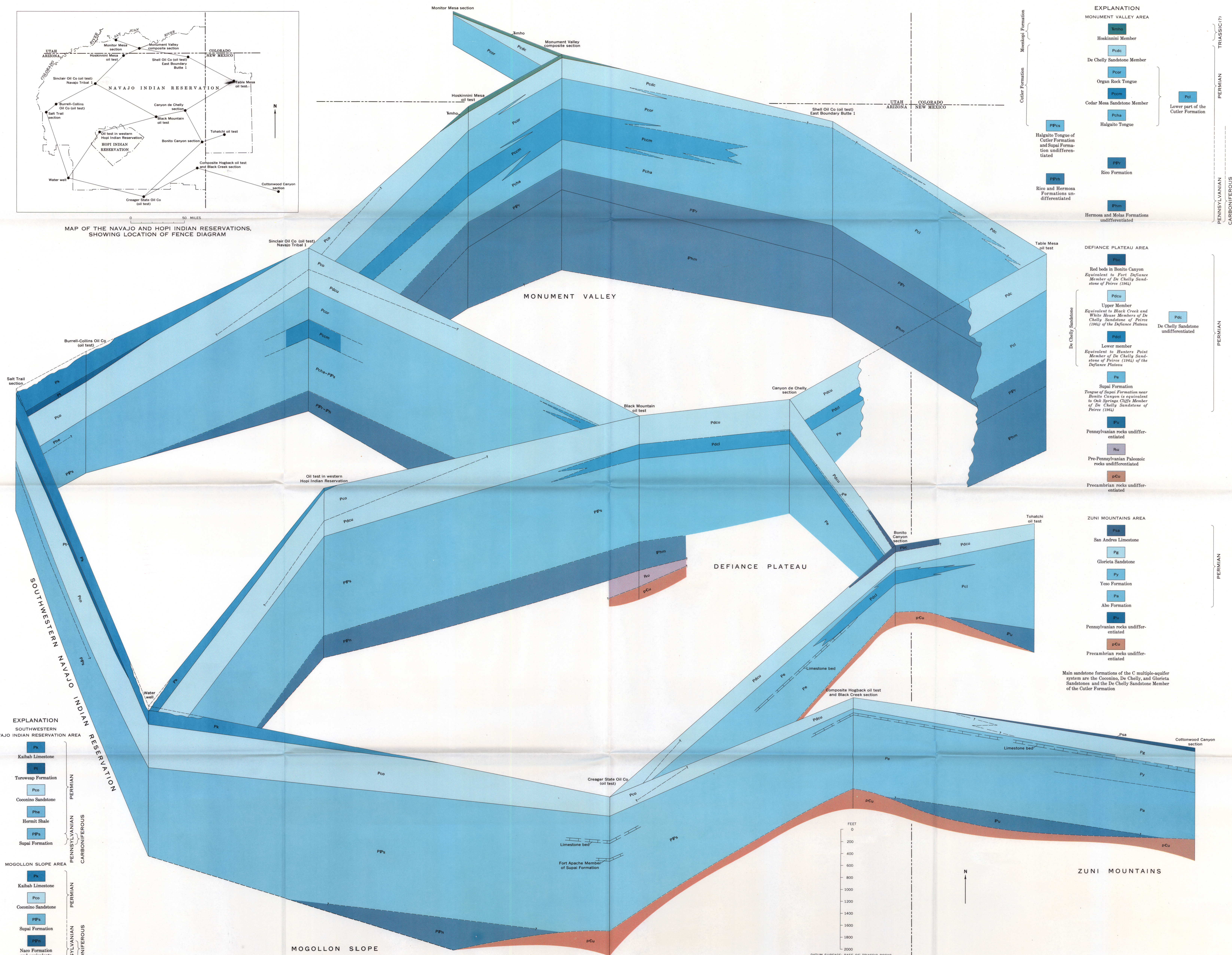
STRATIGRAPHIC FENCE DIAGRAM OF THE PALEOZOIC ROCKS OF THE NAVAJO AND HOPI INDIAN RESERVATIONS, ARIZONA, NEW MEXICO, AND UTAH
