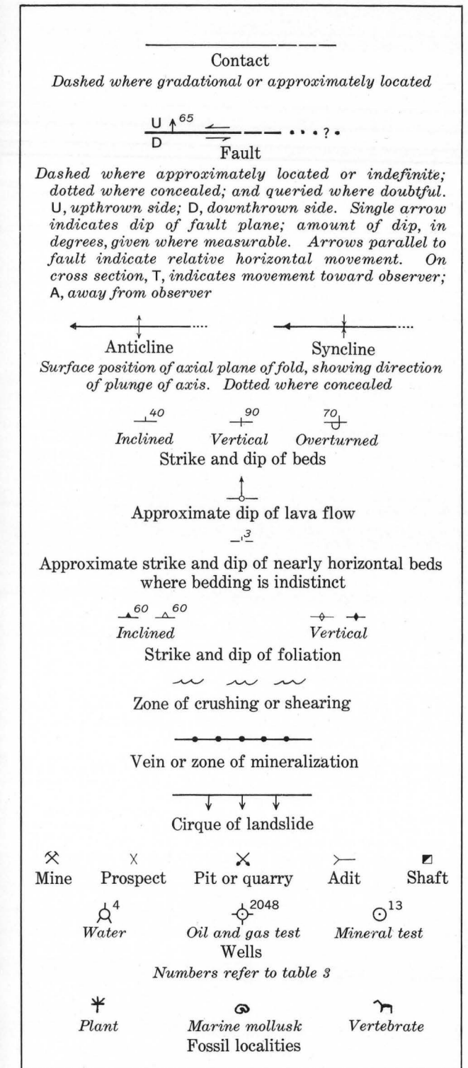
GEOLOGIC MAP SYMBOLS
