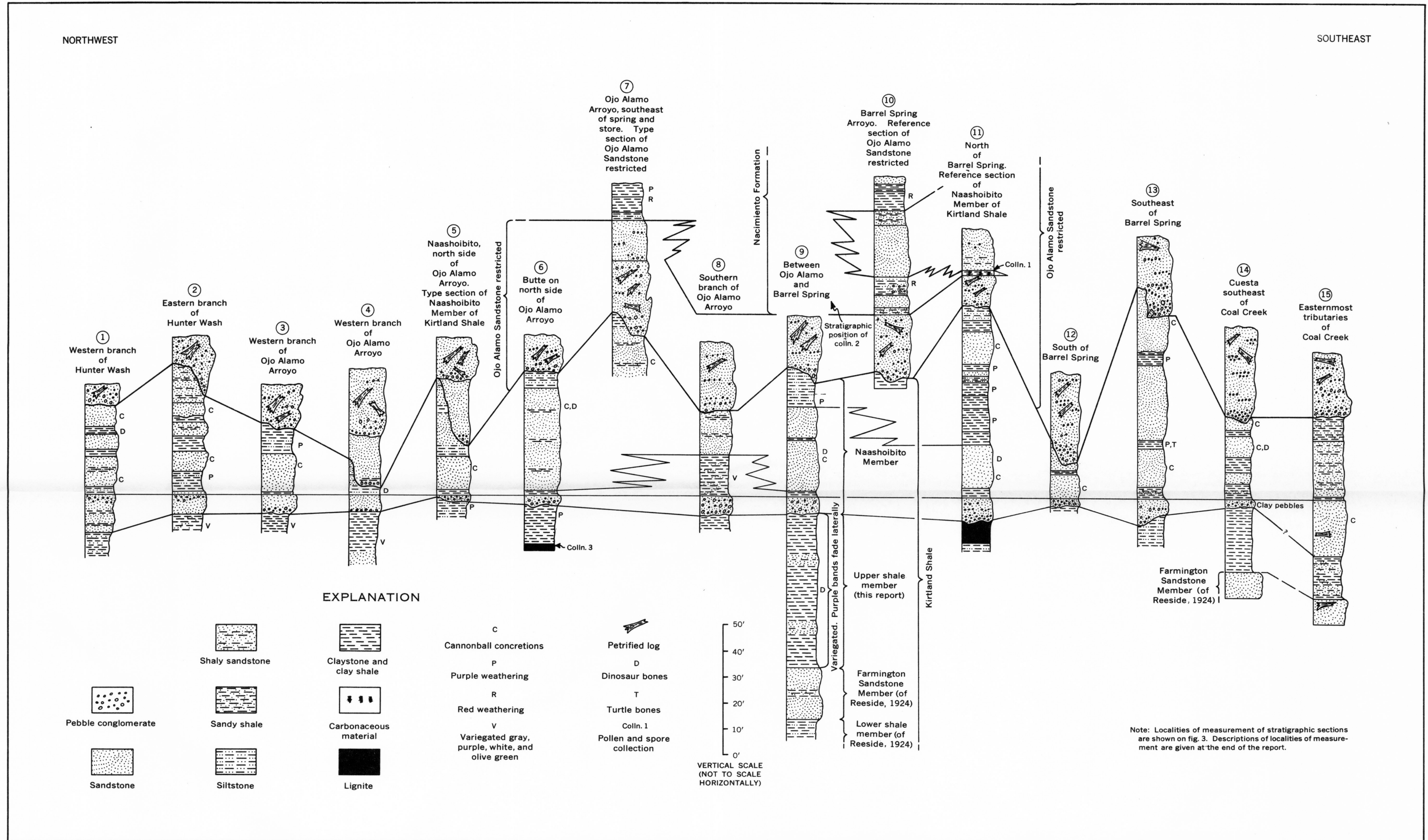
STRATIGRAPHIC SECTIONS OF THE RESTRICTED OJO ALAMO SANDSTONE AND THE OVERLYING AND UNDERLYING ROCKS IN THE TYPE REGION BETWEEN HUNTER WASH AND THE EASTERN FORK OF COAL CREEK, SAN JUAN COUNTY, NEW MEXICO
