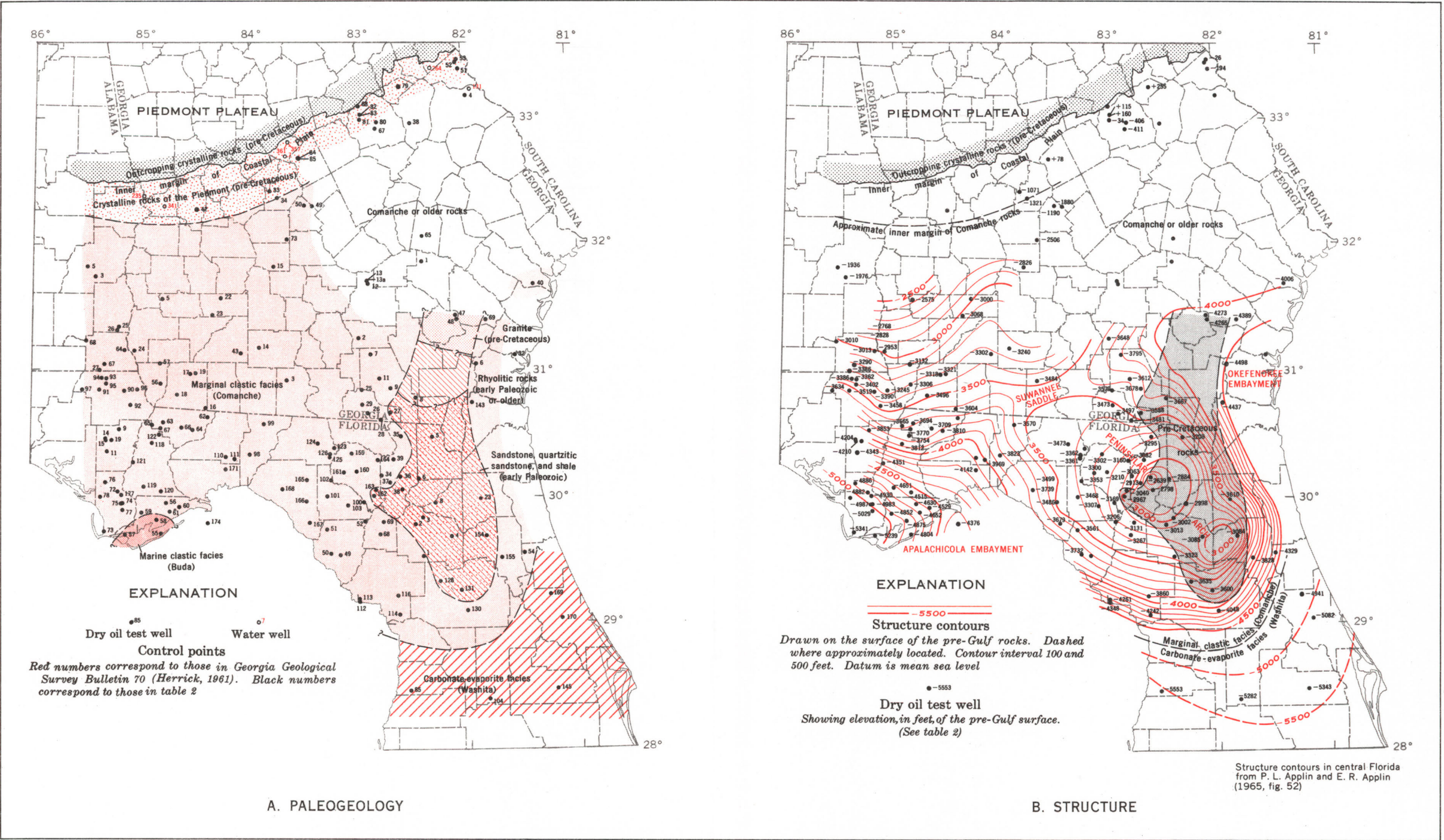
MAPS SHOWING PALEO GEOLOGY AND STRUCTURE OF THE PRE-GULF SURFACE IN NORTHERN FLORIDA AND SOUTHERN GEORGIA
