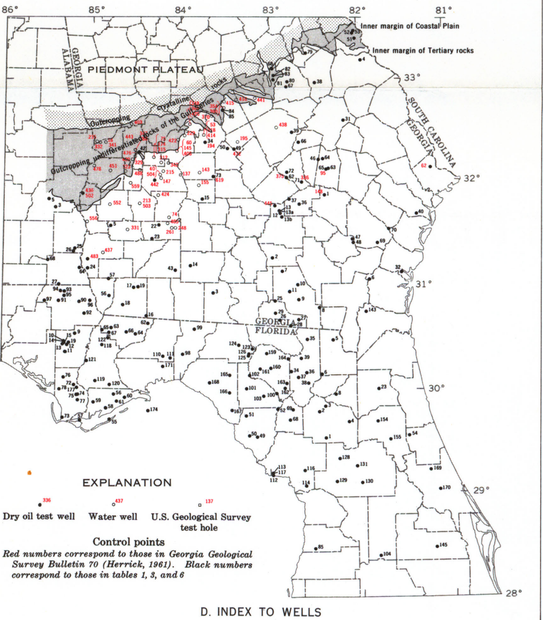
MAPS SHOWING GEOLOGY AND STRUCTURE OF THE SURFACE AND TOTAL THICKNESS OF THE GULF SERIES IN NORTHERN FLORIDA AND SOUTHERN GEORGIA
