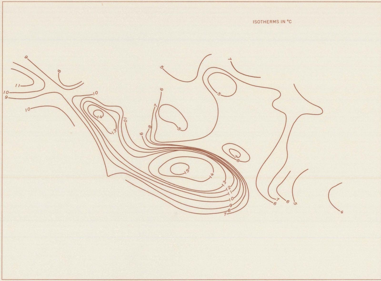
Bottom isotherms for the warmest part of the year (mid-September through October), Nova Scotia to Long Island (from Schopf, 1967). For use with plates 7-30, 55-59, and 61-69.
