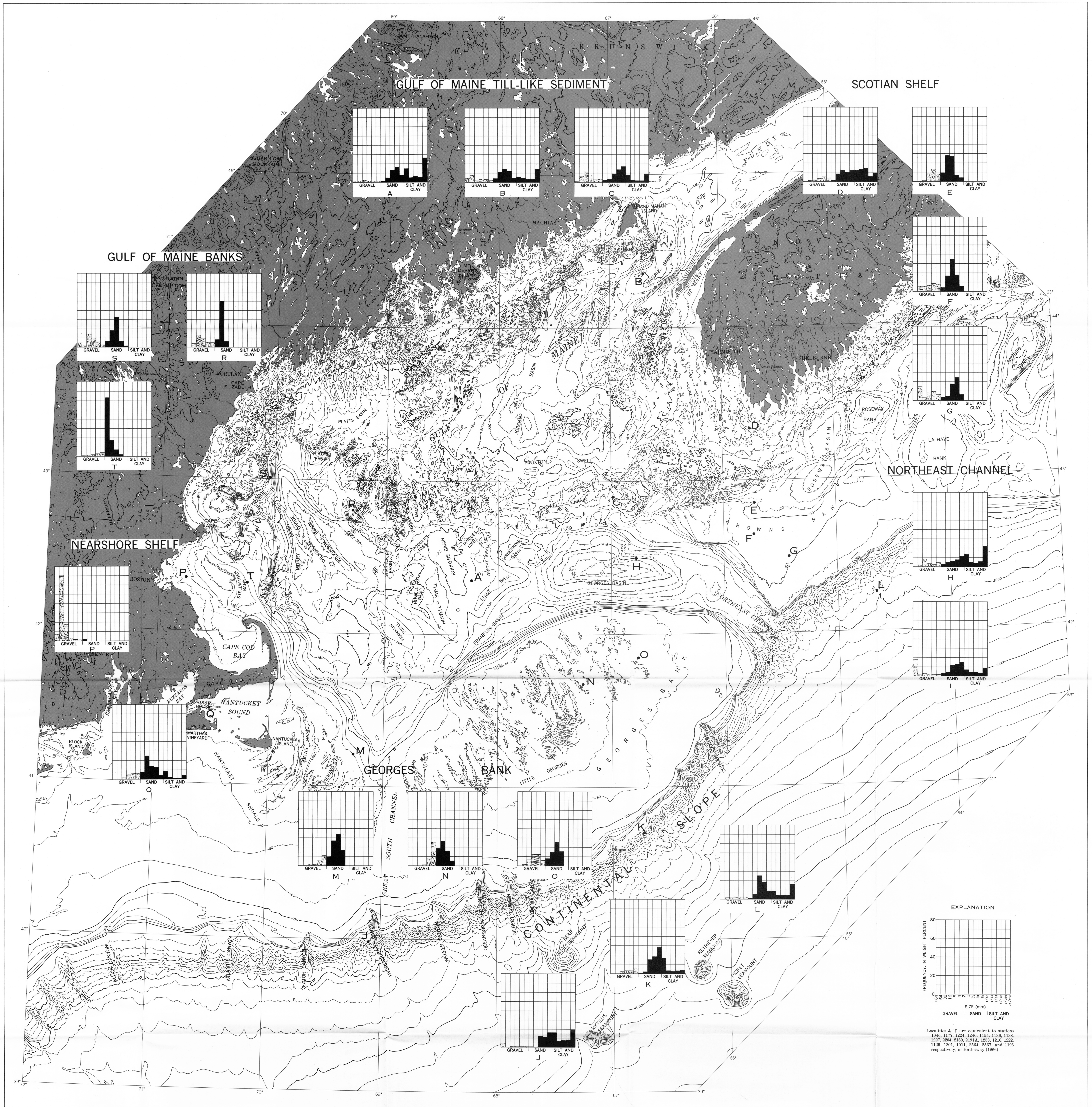
BATHYMETRIC MAP OF THE CONTINENTAL MARGIN OFF NEW ENGLAND AND NOVA SCOTIA SHOWING LOCATIONS AND HISTOGRAMS OF SELECTED GRAVELLY SAMPLES
