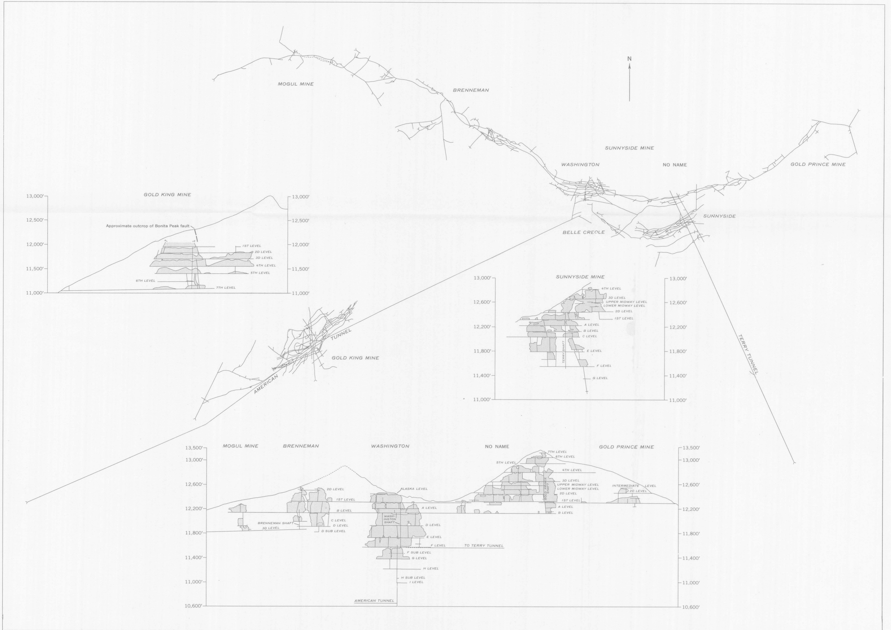
PLAN MAP AND VERTICAL PROJECTIONS OF MINE WORKINGS AND STOPES IN THE SUNNYSIDE AND GOLD KING MINES, EUREKA MINING DISTRICT, SAN JUAN MOUNTAINS, COLORADO
