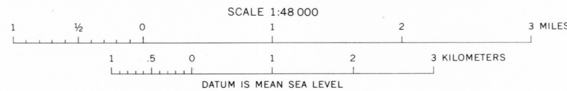
STRUCTURAL SECTIONS IN GREENWOOD QUADRANGLE, SEBASTIAN COUNTY, ARKANSAS, AND LE FLORE COUNTY, OKLAHOMA
