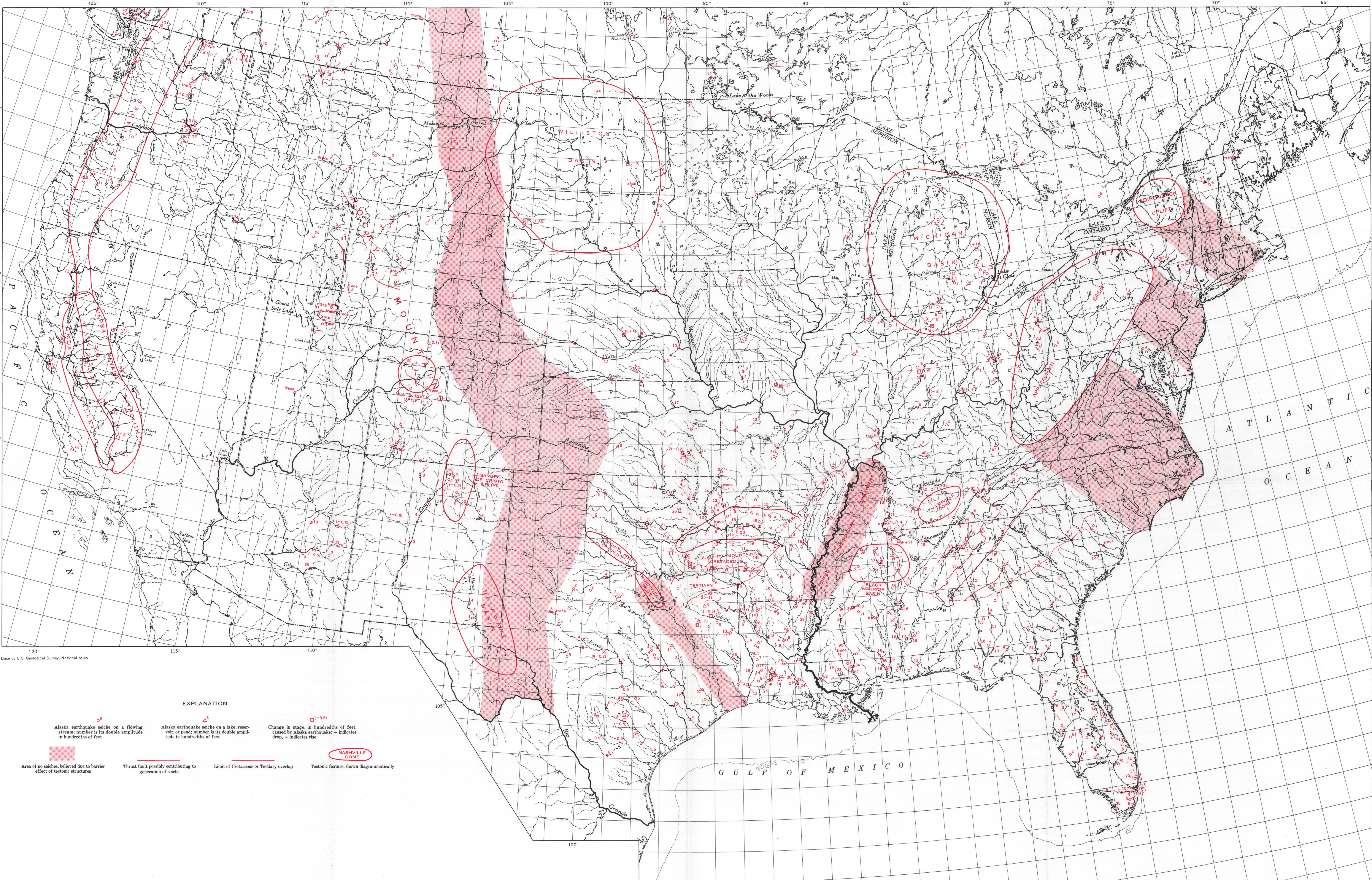
MAP OF THE CONTERMINOUS UNITED STATES AND SOUTHERN CANADA SHOWING OCCURRENCE OF SEICHES FROM THE ALASKA EARTHQUAKE AND THEIR RELATION TO MAJOR TECTONIC FEATURES
