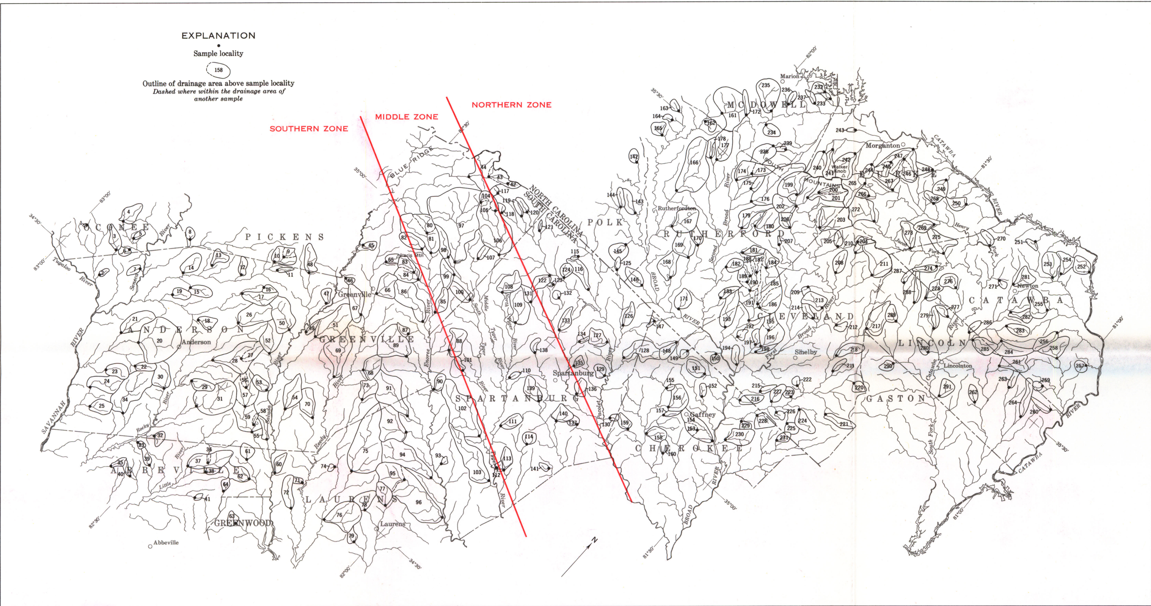
A. SAMPLE LOCALITIES AND GEOGRAPHIC SUBDIVISION OF MAGNETITE SEPARATES
