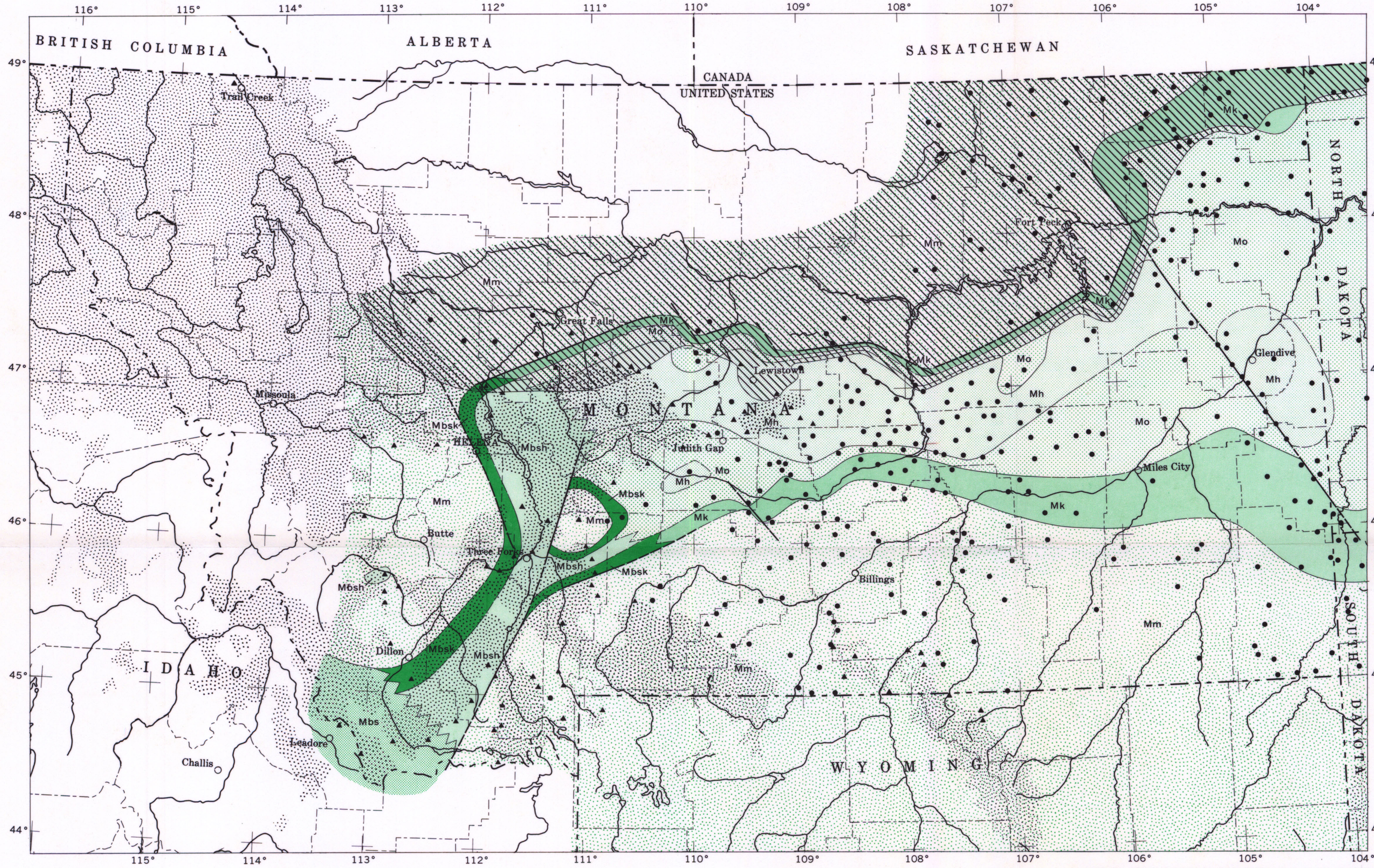
PALEOGEOLOGIC MAP SHOWING DISTRIBUTION OF BIG SNOWY AND MADISON GROUPS IN MONTANA
