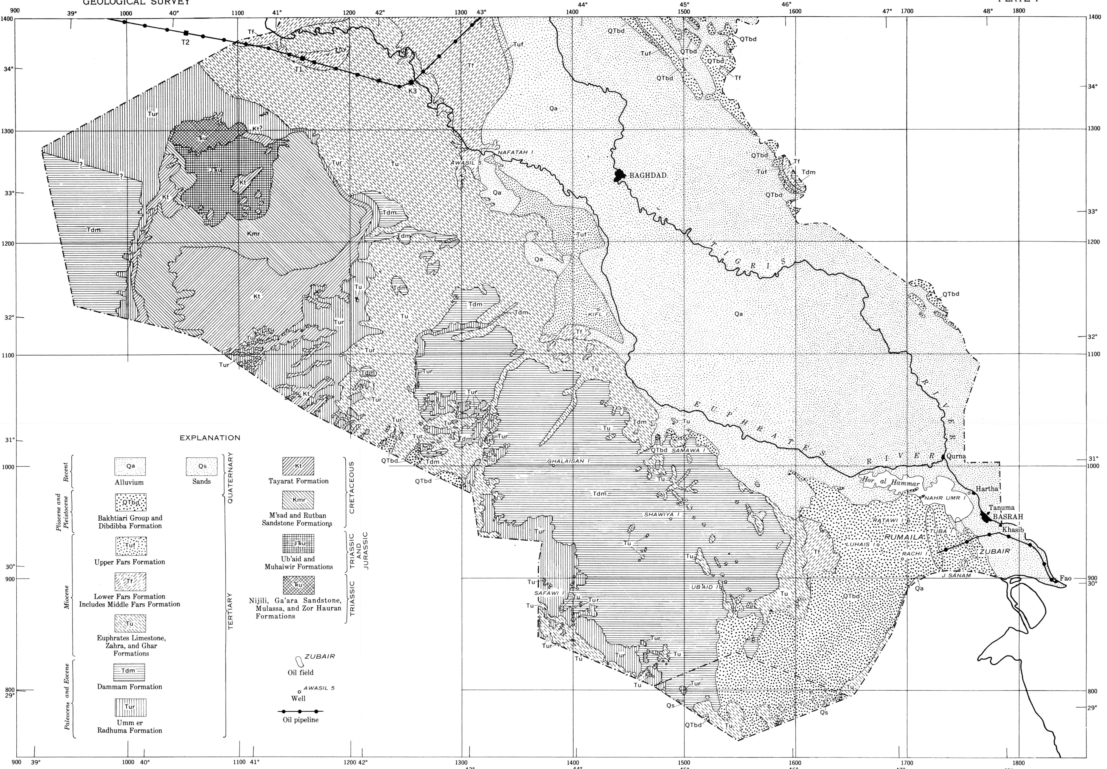
GENERALIZED GEOLOGIC MAP OF CENTRAL AND SOUTHERN IRAQ
