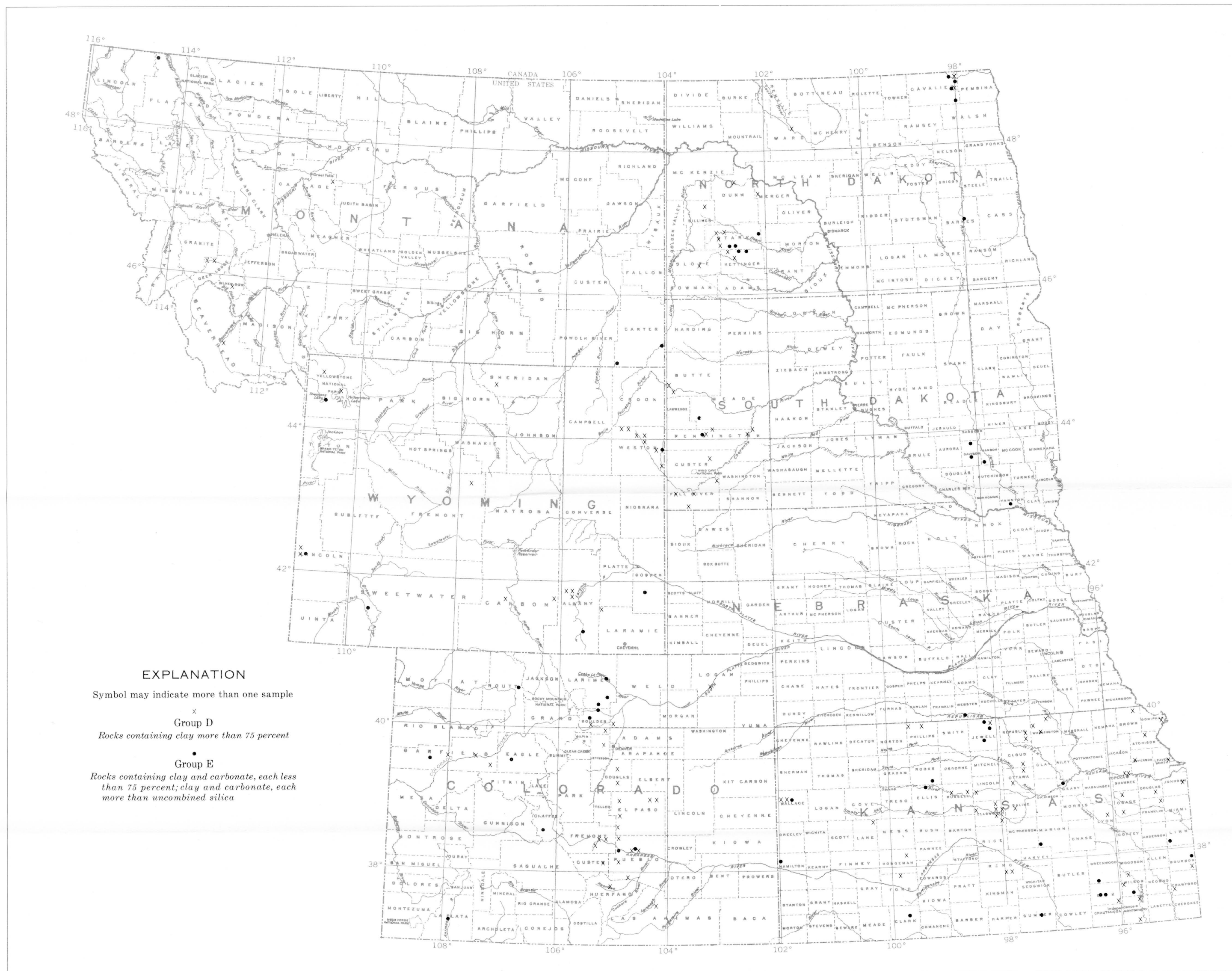
MAP SHOWING SAMPLE LOCALITIES OF ROCKS IN GROUPS D AND E COMMON- AND MIXED-ROCK CATEGORIES
