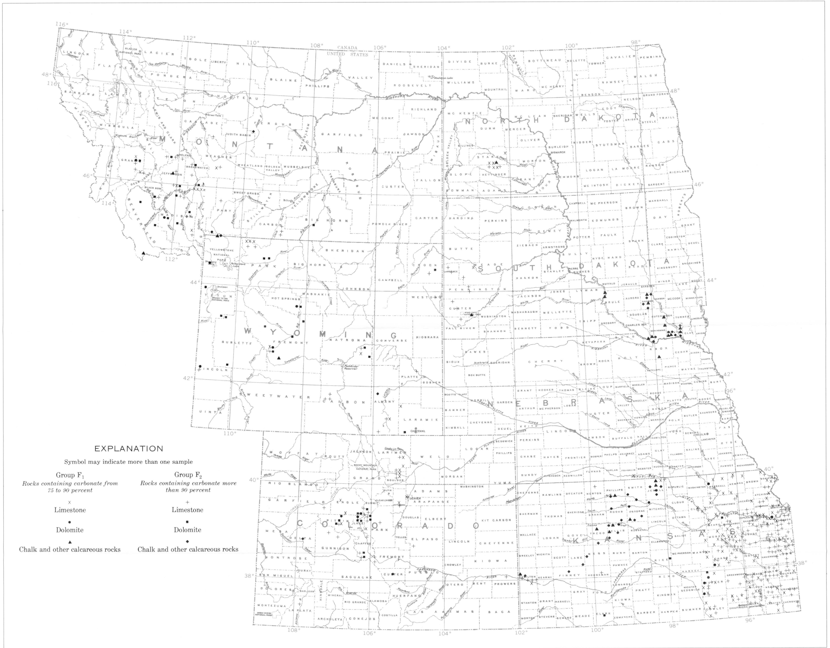
MAP SHOWING SAMPLE LOCALITIES OF LIMESTONE, DOLOMITE, AND CHALK IN GROUPS F 1 AND F 2 COMMON- AND MIXED-ROCK CATEGORIES
