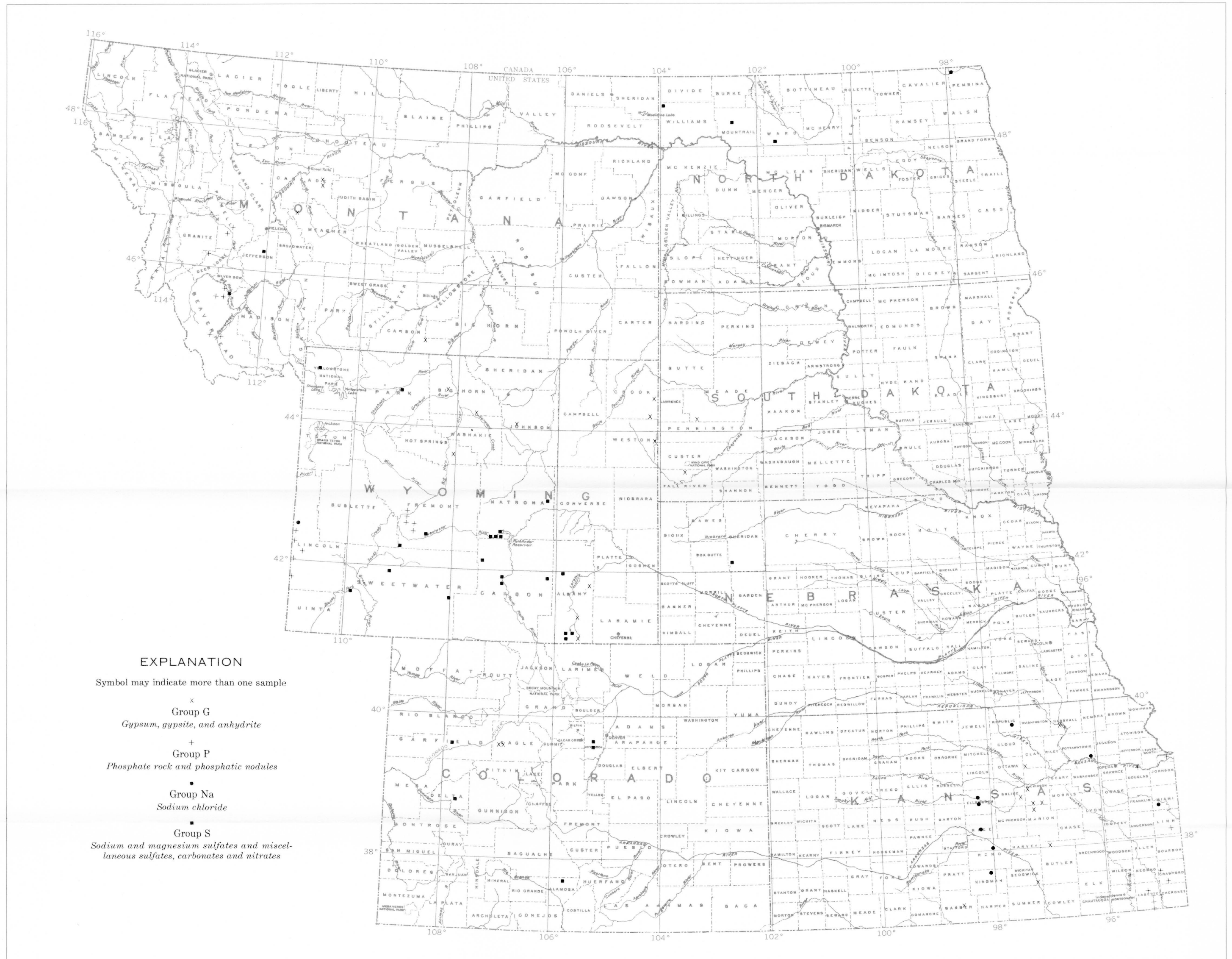
MAP SHOWING SAMPLE LOCALITIES OF SULFATE-, PHOSPHATE-, AND CHLORIDE-BEARING ROCKS SPECIAL-ROCK CATEGORY
