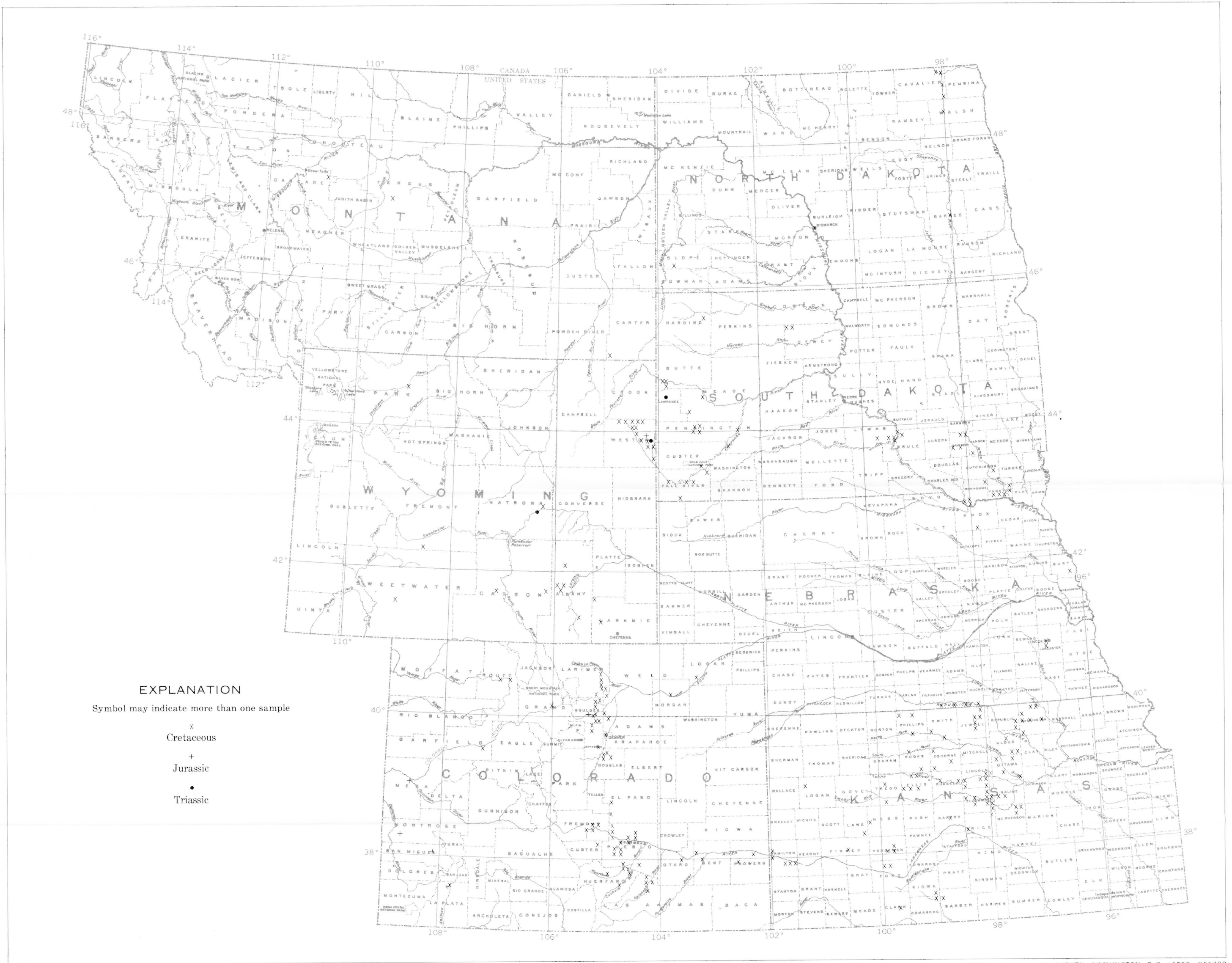
MAP SHOWING SAMPLE LOCALITIES OF ROCKS OF TRIASSIC, JURASSIC, AND CRETACEOUS AGES COMMON- AND MIXED-ROCK CATEGORIES
