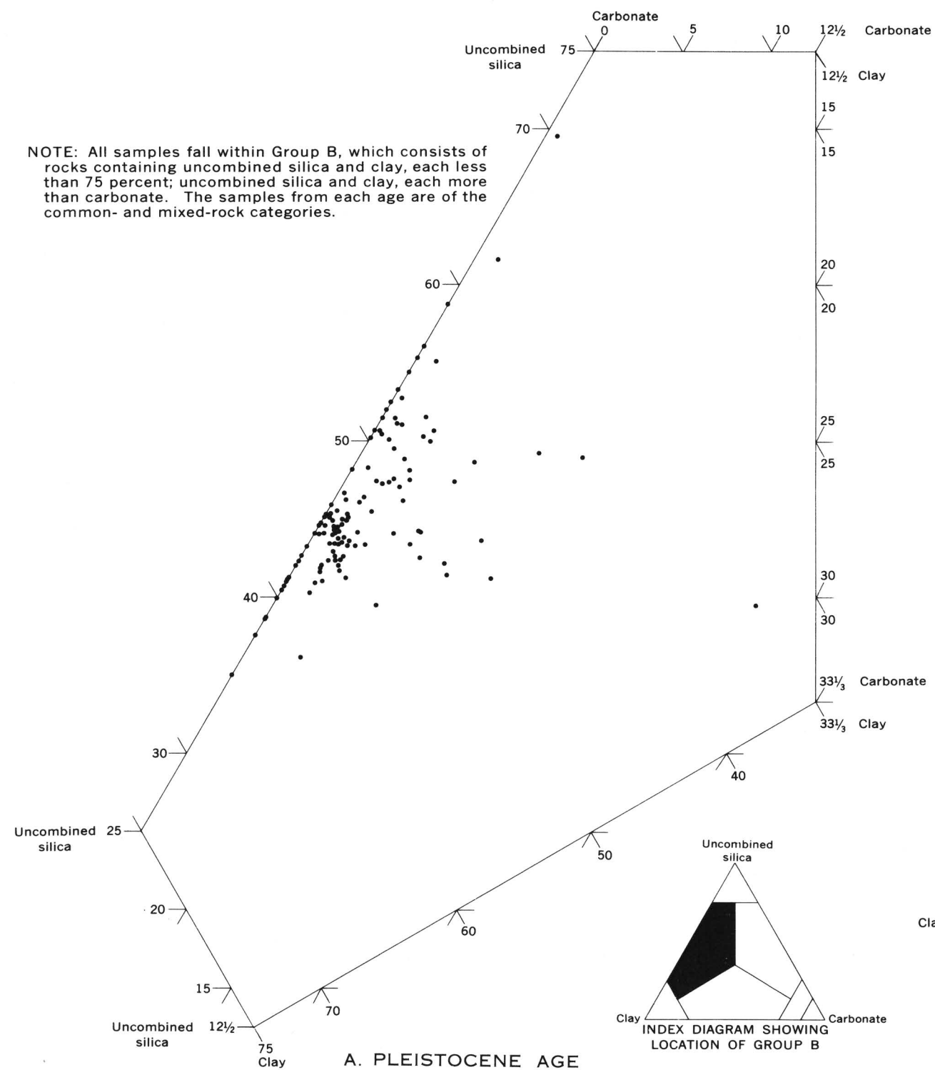
DIAGRAMS SHOWING DISTRIBUTION AMONG COMPOSITIONAL GROUPS OF ANALYSES OF MATERIALS OF QUATERNARY AGE FROM THE NORTHERN ROCKY MOUNTAINS AND GREAT PLAINS REGION
