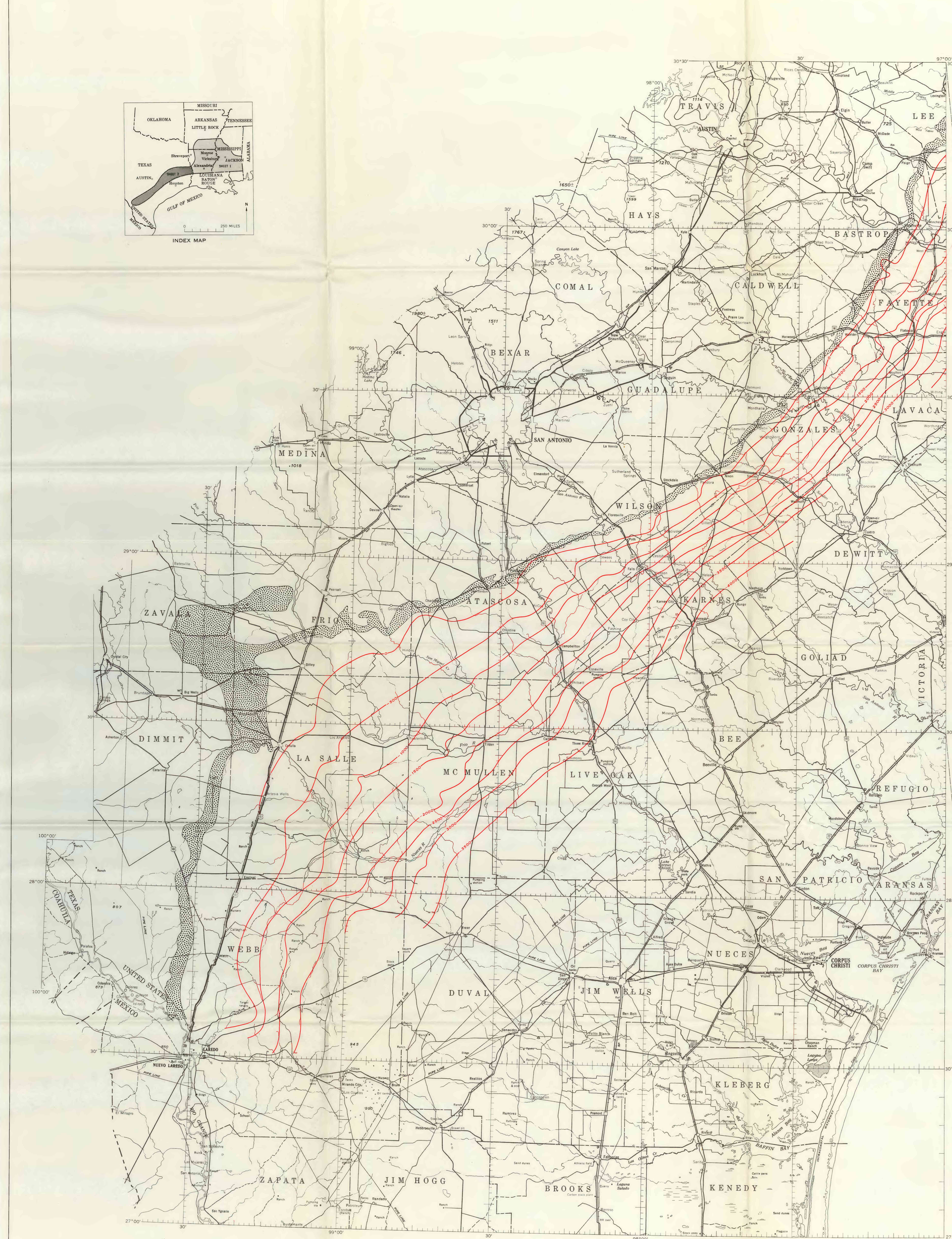
STRUCTURE-CONTOUR MAP ON THE BASE OF THE SPARTA SAND IN ARKANSAS, LOUISIANA, MISSISSIPPI, AND TEXAS
