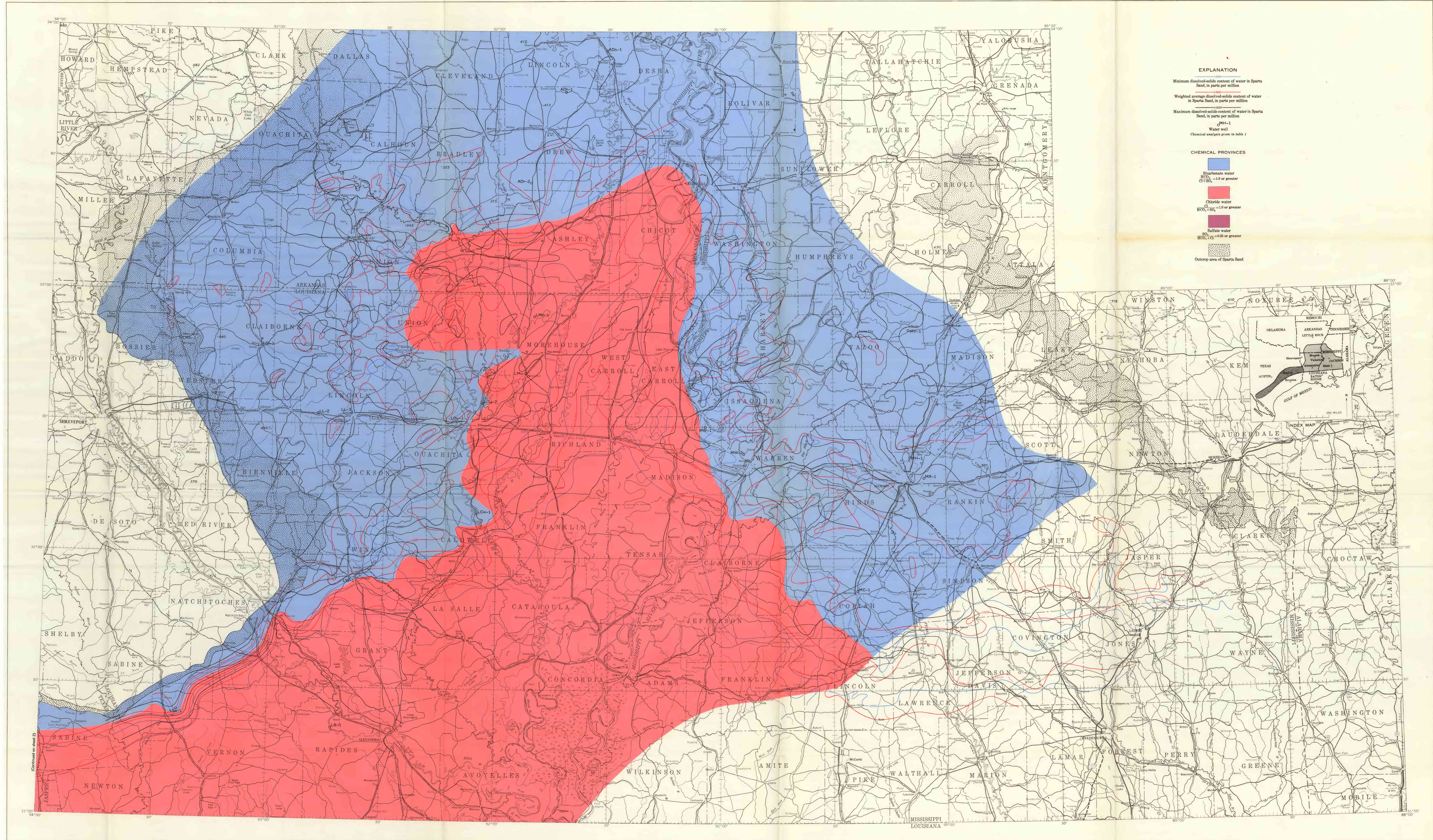
MAP SHOWING DISSOLVED-SOLIDS CONTENT AND CHEMICAL PROVINCES OF WATER IN THE SPARTA SAND IN ARKANSAS, LOUISIANA, MISSISSIPPI, AND TEXAS
