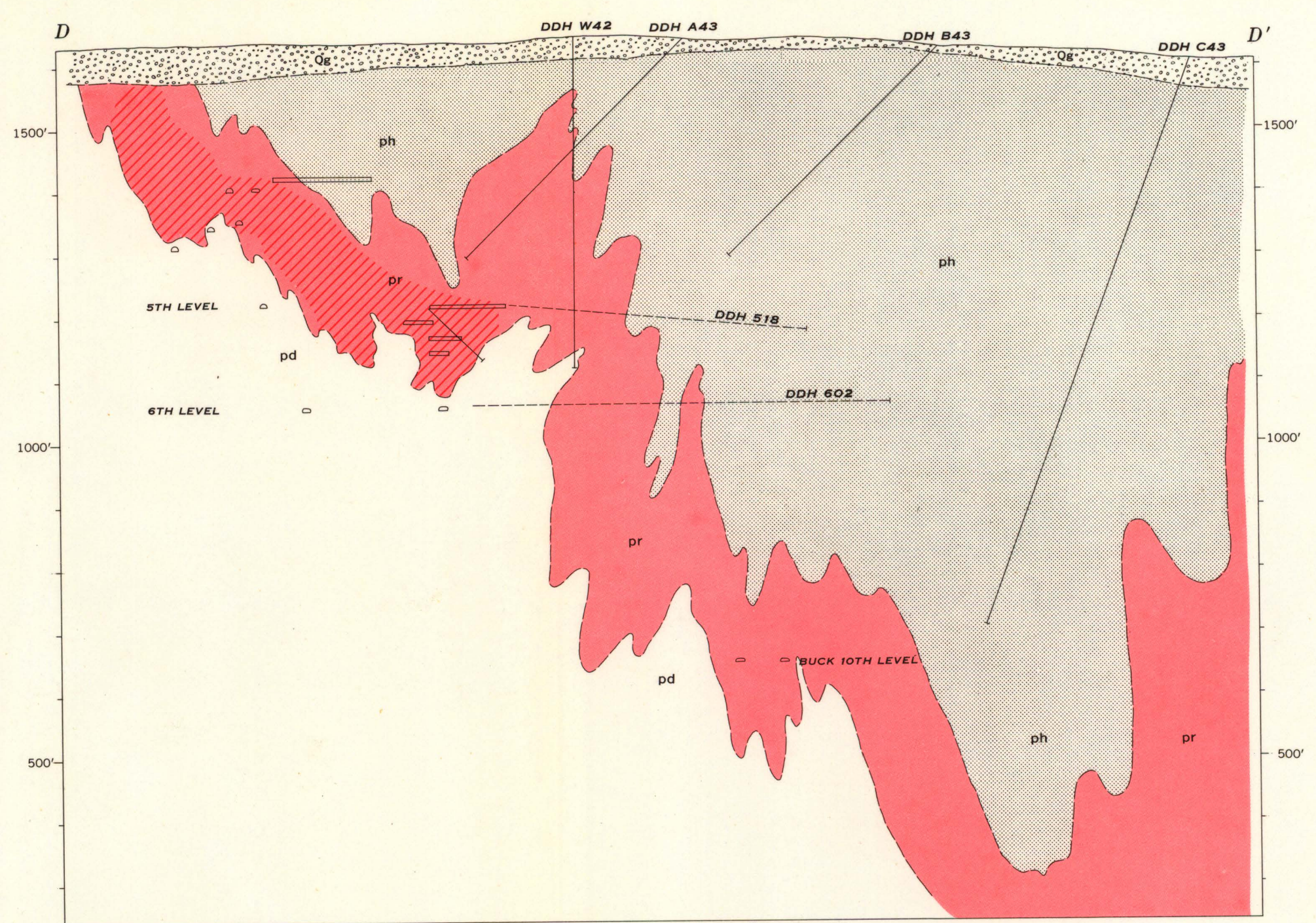
D-D' SECTION THROUGH WORKINGS OF THE ZIMMERMAN MINE
