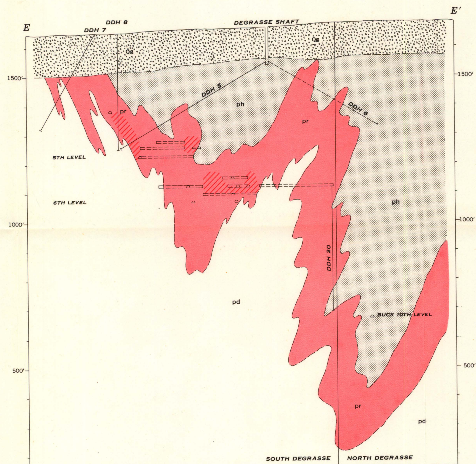
E-E' SECTION THROUGH DEGRASSE SHAFT AND EASTERN WORKINGS OF ZIMMERMAN AND BUCK MINES
