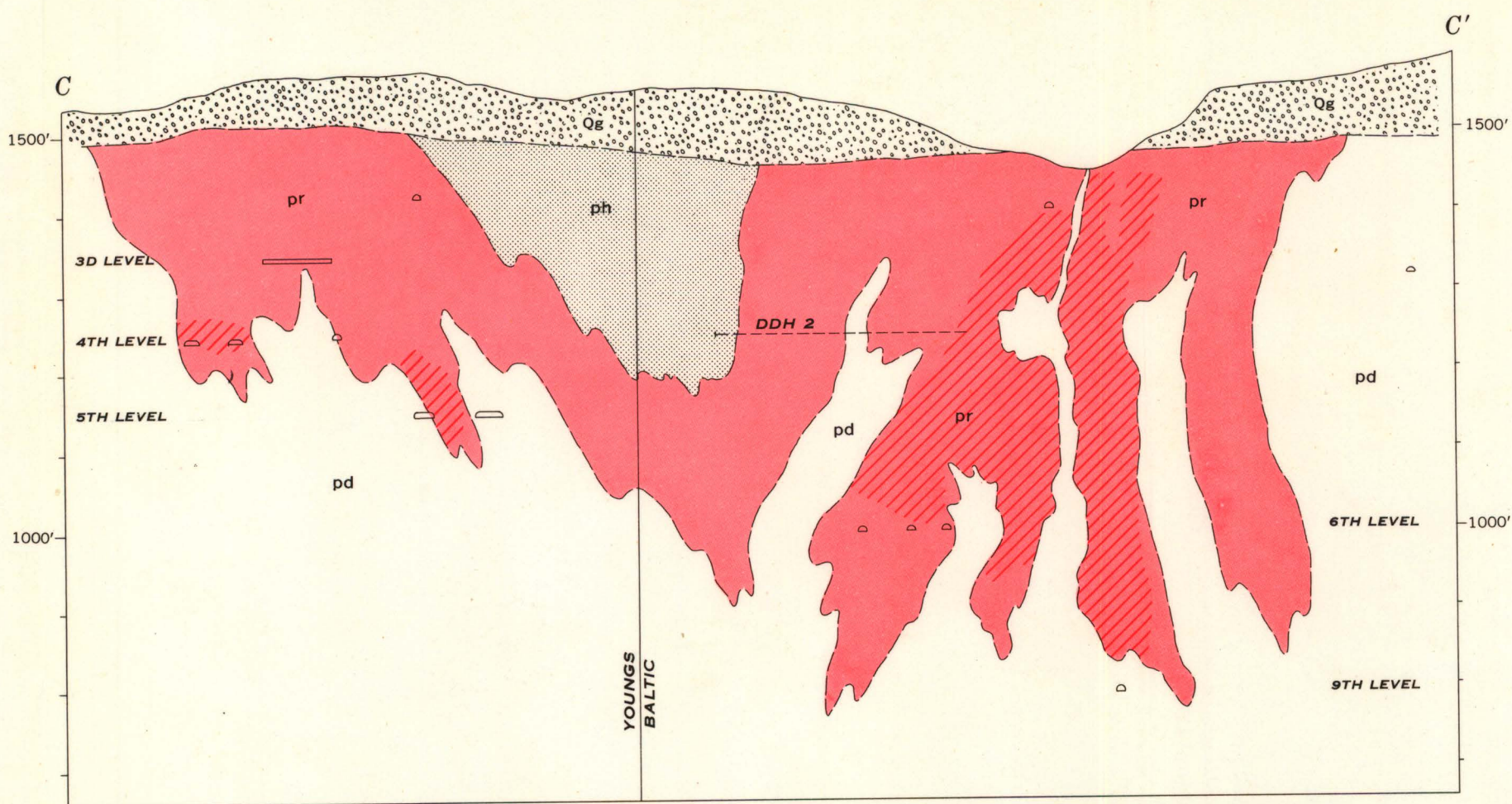
C-C' SECTION THROUGH WORKINGS OF THE YOUNGS AND BALTIC MINES
