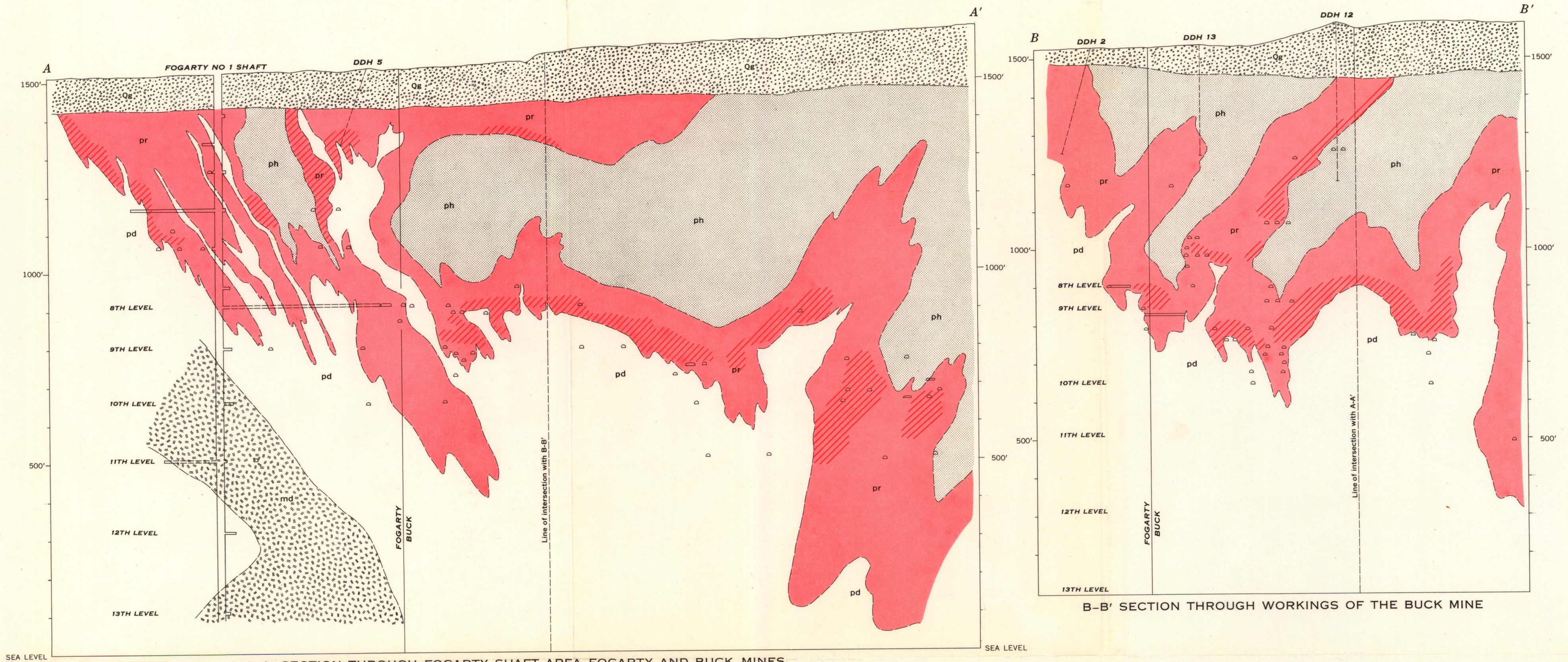
A-A' SECTION THROUGH FOGARTY SHAFT AREA, FOGARTY AND BUCK MINES
