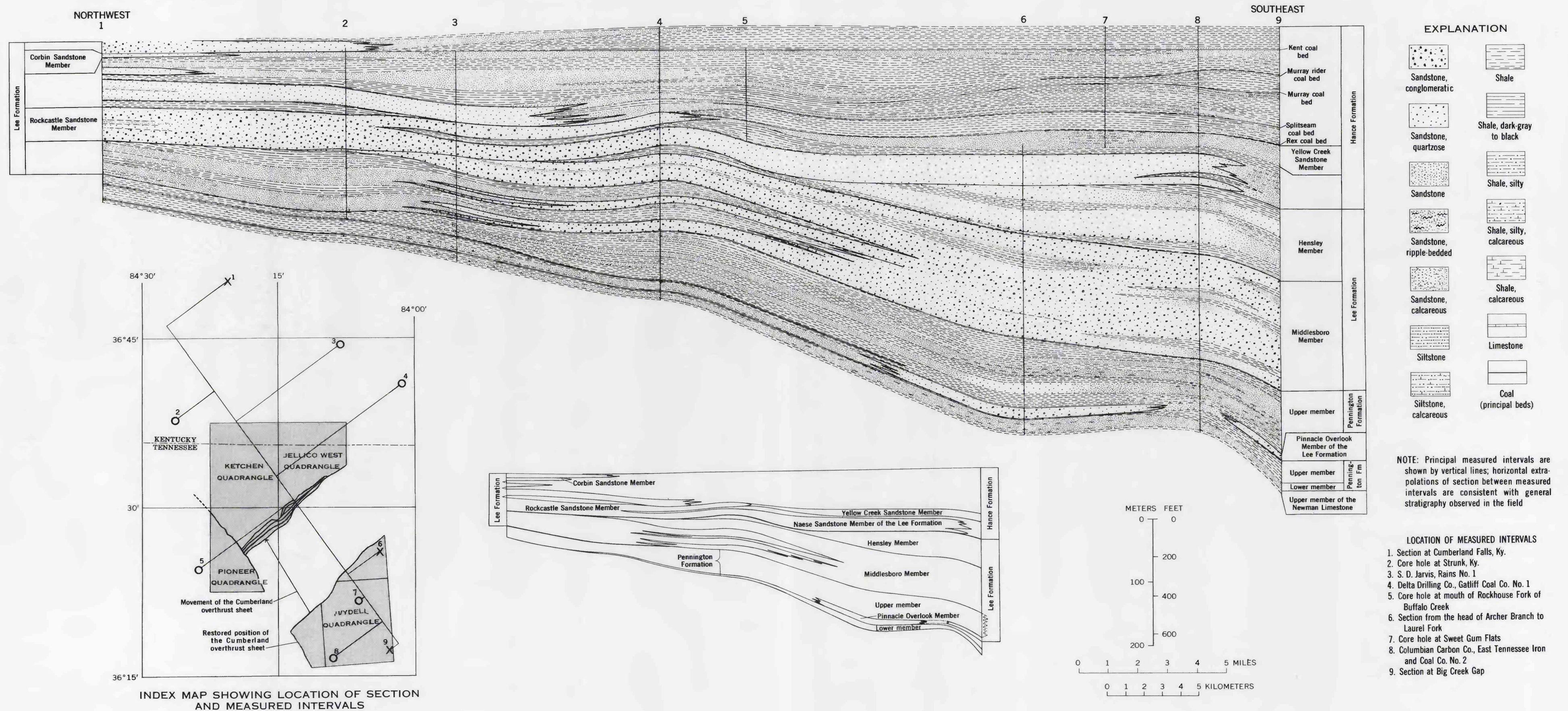
STRATIGRAPHIC SECTION ILLUSTRATING INTERRELATION OF THE PENNINGTON, LEE, AND HANCE FORMATIONS, TENNESSEE AND KENTUCKY
