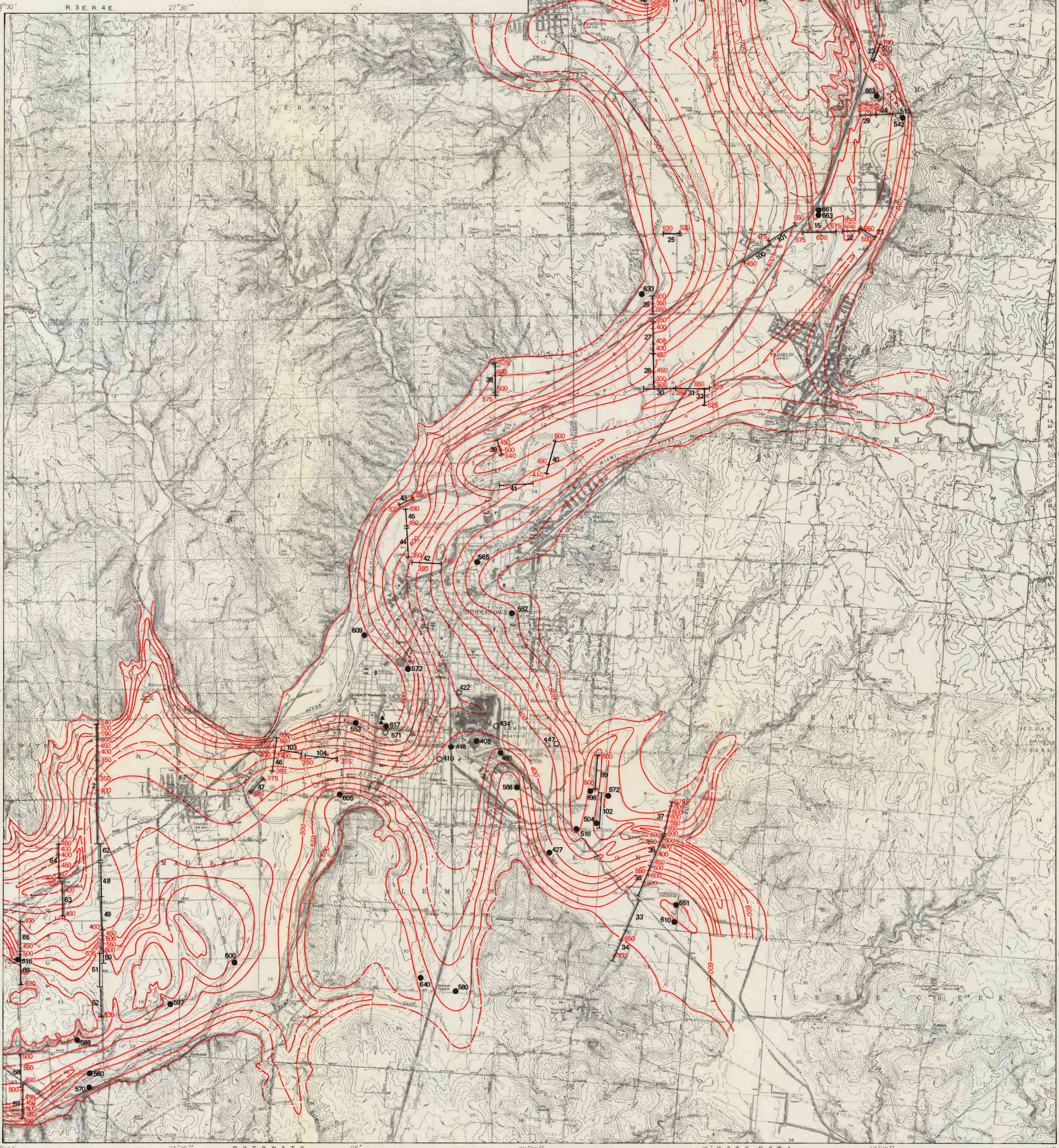
MAP SHOWING CONTOURS ON THE BEDROCK SURFACE AND LOCATION OF WELLS AND SEISMIC LINES, LOWER GREAT MIAMI RIVER VALLEY, OHIO
