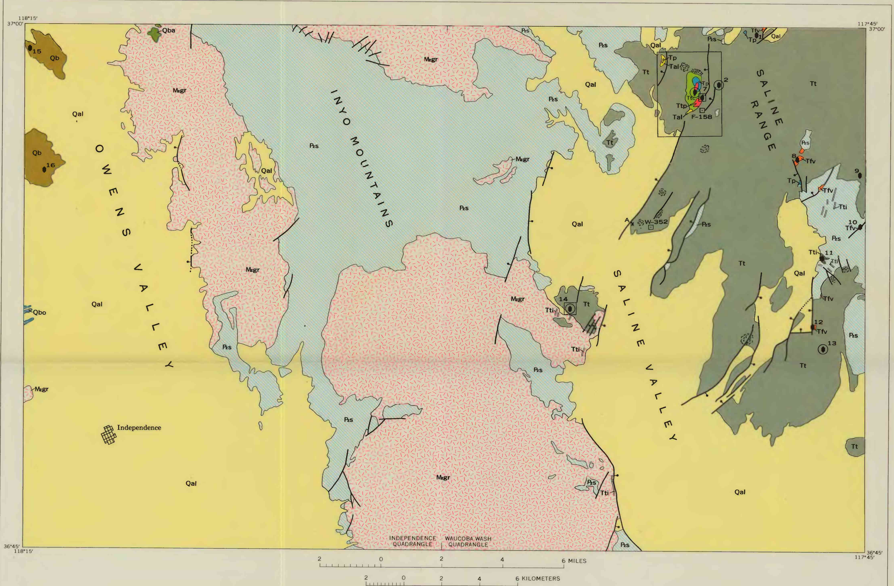
A. GENERALIZED GEOLOGIC MAP
