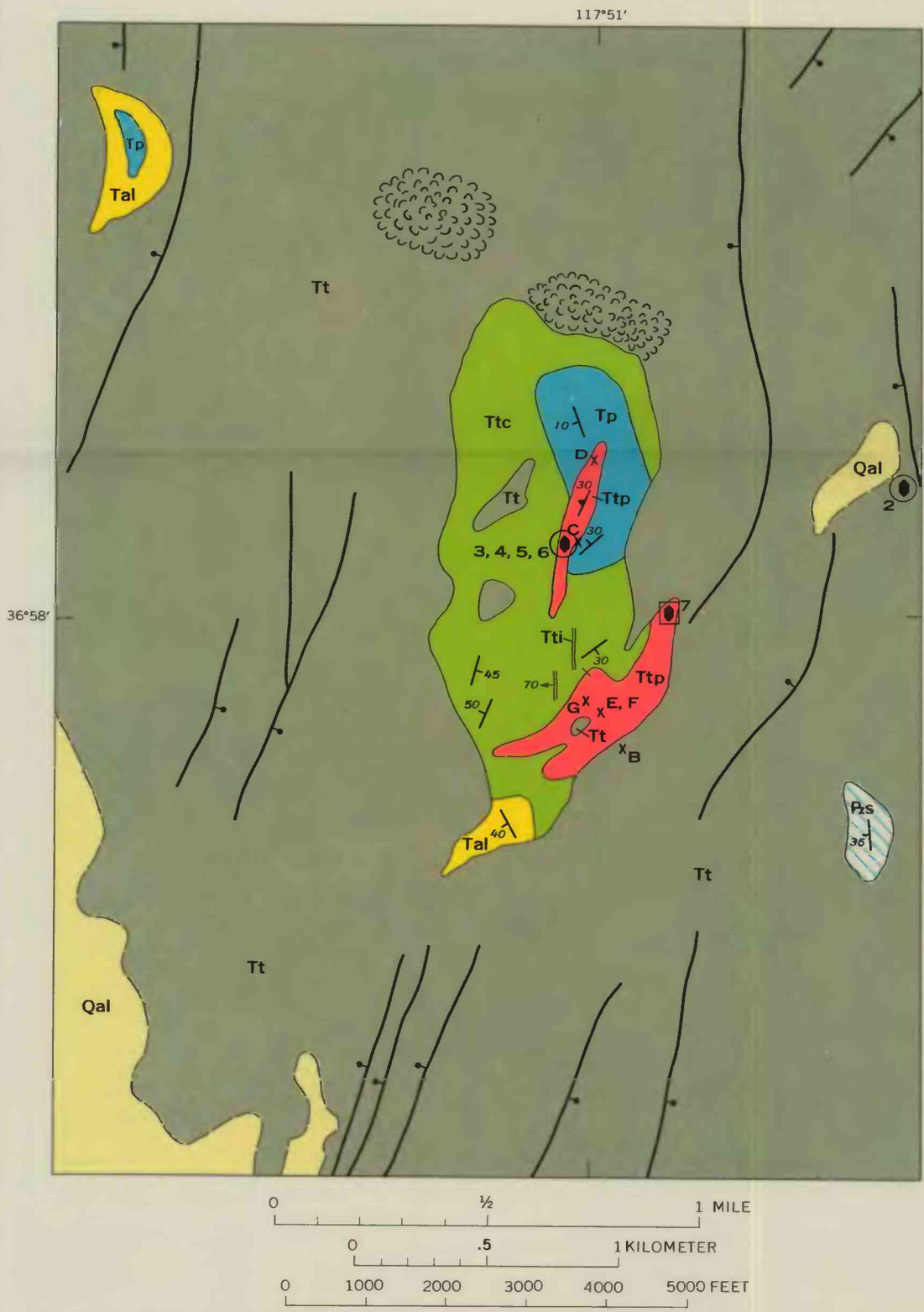
B. WINDOW IN TRACHYANDESITE VOLCANIC FIELD, SALINE RANGE
