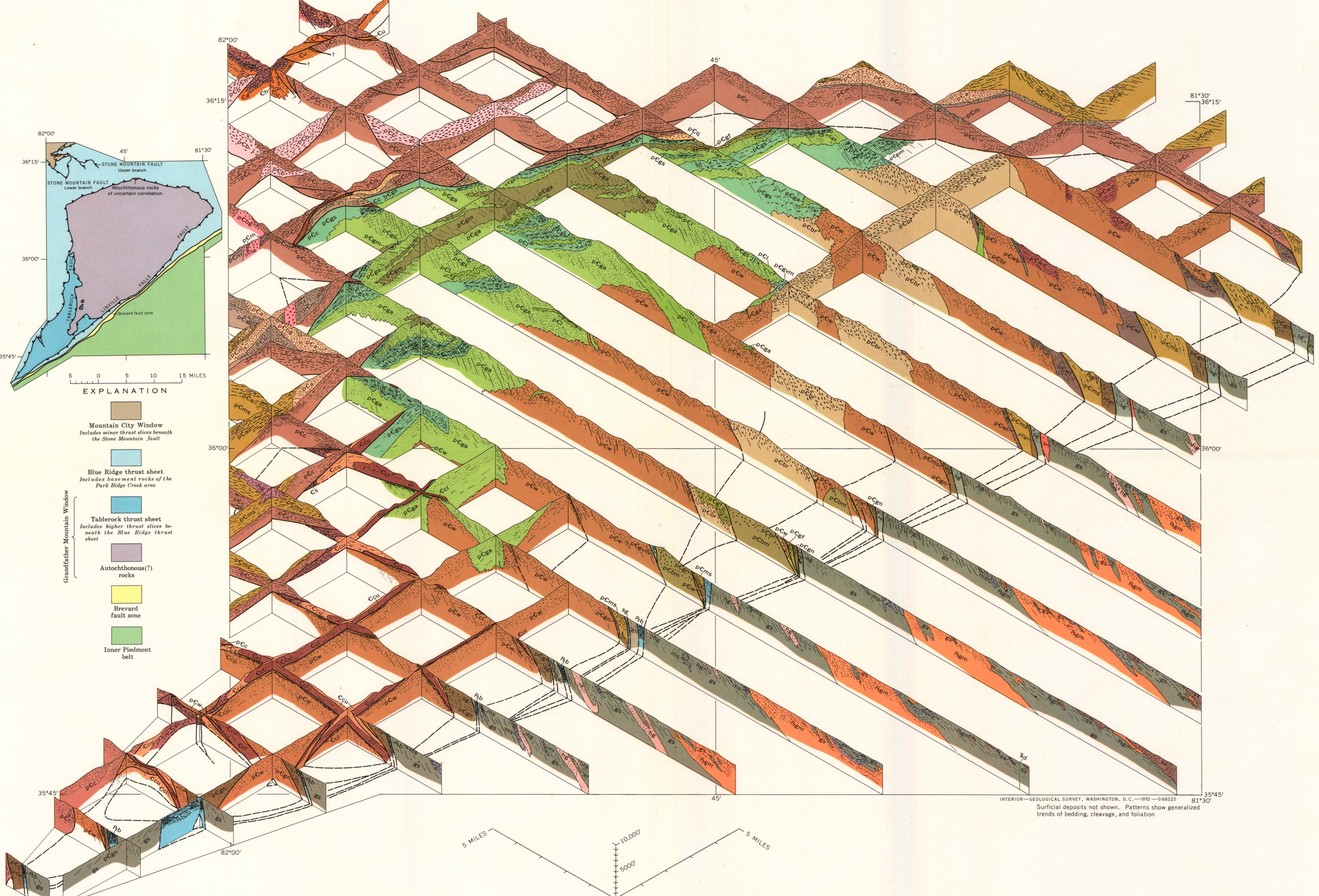
EXPLANATION, FENCE DIAGRAM, AND GENERALIZED TECTONIC MAP OF THE GRANDFATHER MOUNTAIN WINDOW AND VICINITY, NORTH CAROLINA AND TENNESSEE
