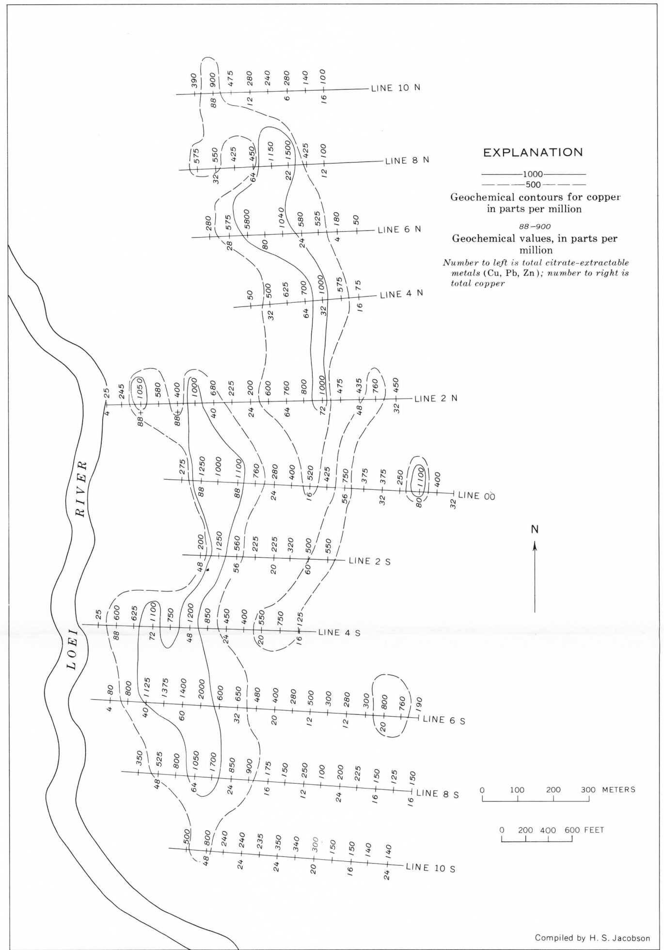
B. GEOCHEMICAL SOIL SURVEY
