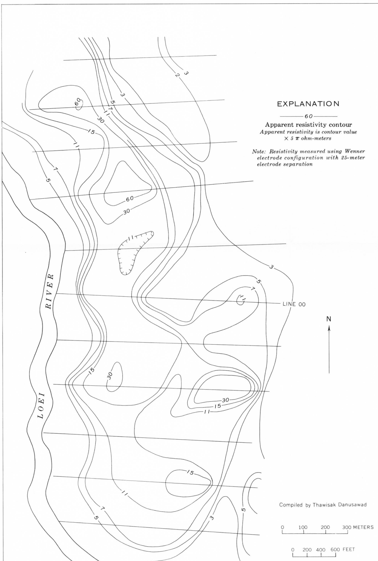
C. RESISTIVITY SURVEY
