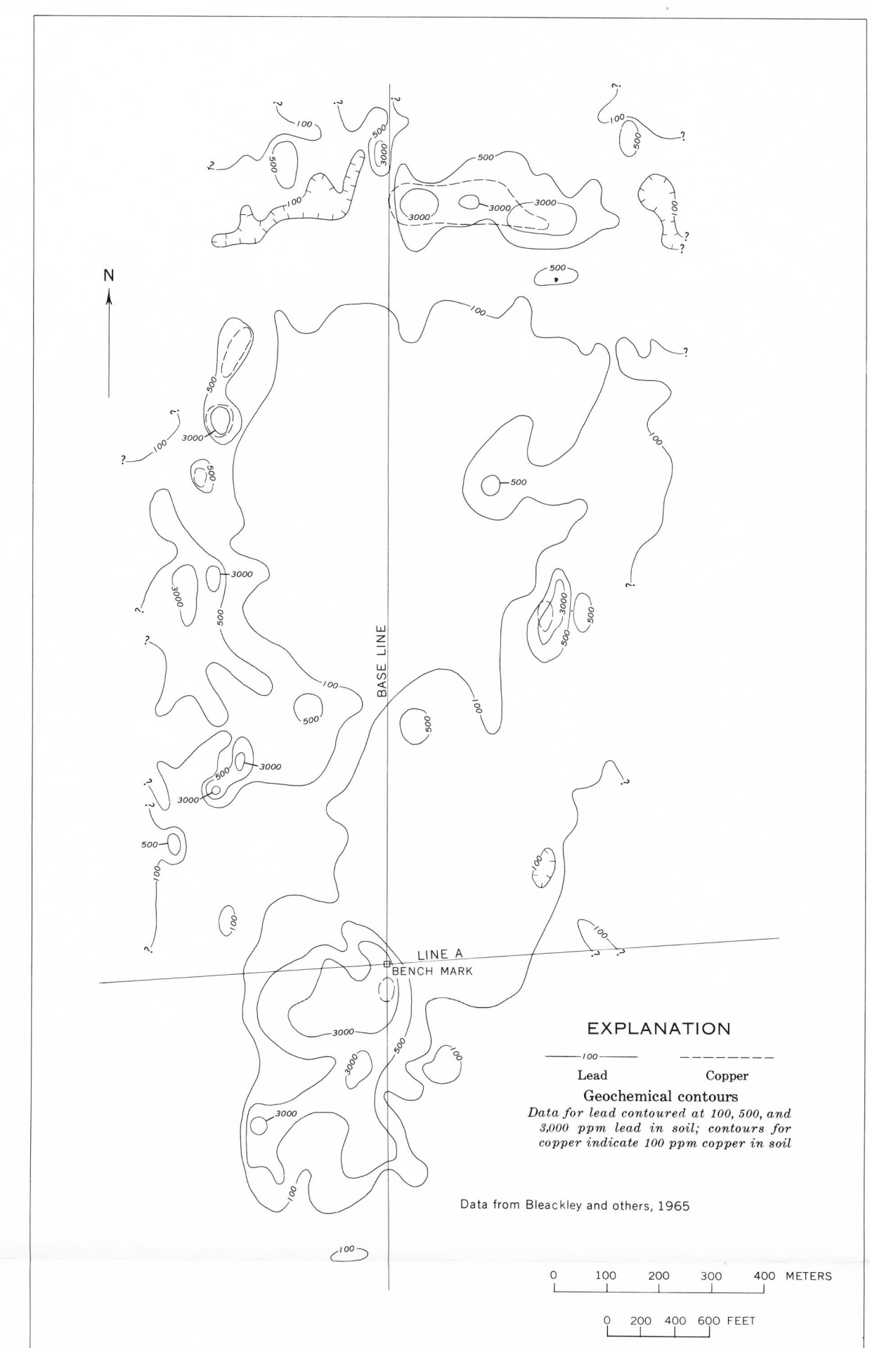
C. GEOCHEMICAL MAP (LEAD AND COPPER)
