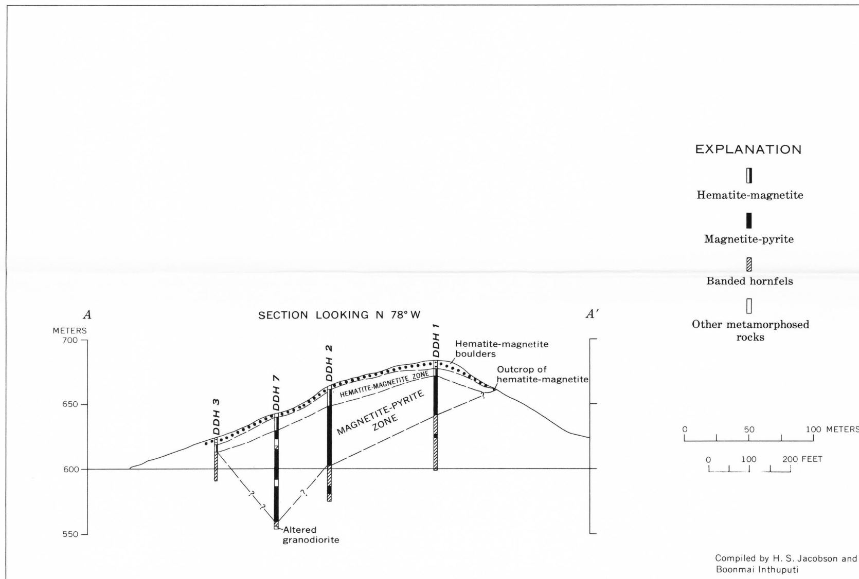
C. GEOLOGIC CROSS SECTION A-A'
