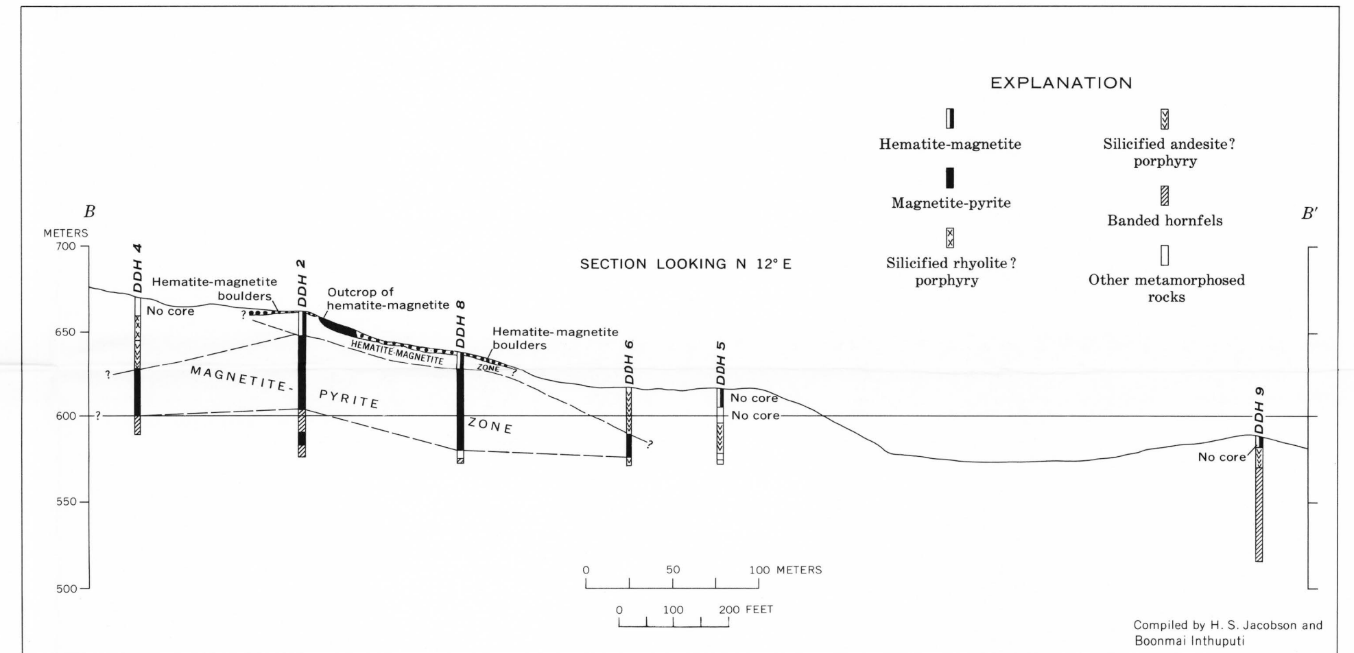
D. GEOLOGIC CROSS SECTION B-B'
