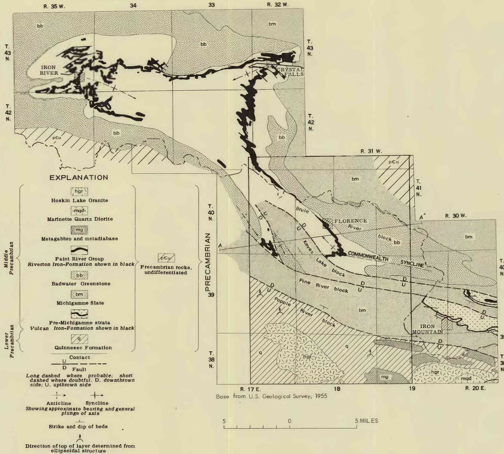
GENERALIZED GEOLOGIC MAP AND SECTIONS SHOWING MAJOR STRUCTURAL FEATURES OF THE FLORENCE AREA, WISCONSIN
