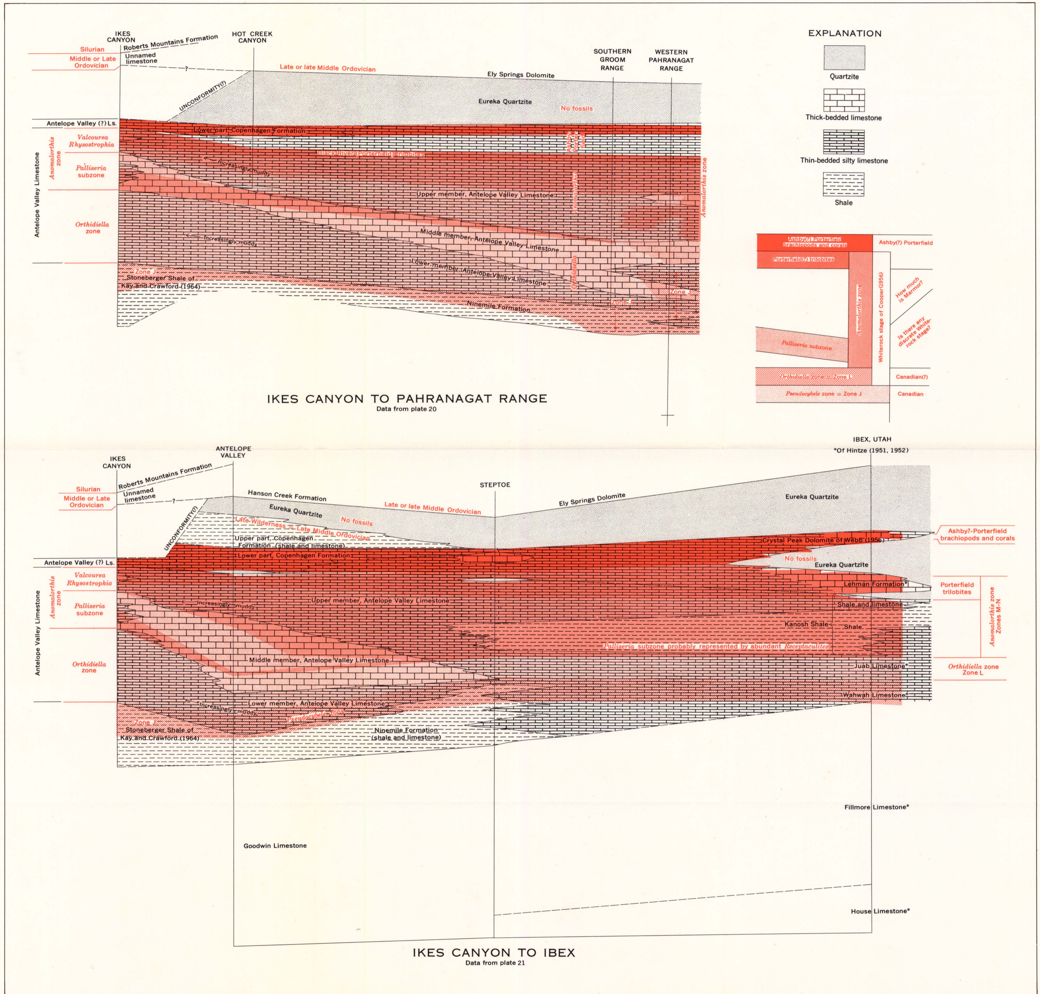
IDEALIZED STRATIGRAPHIC DIAGRAMS SHOWING FOSSIL ZONES RELATIVE TO ORDOVICIAN UNITS FROM THE PAHRANAGAT RANGE TO IKES CANYON AND FROM IBEX, UTAH, TO IKES CANYON, NEVADA
