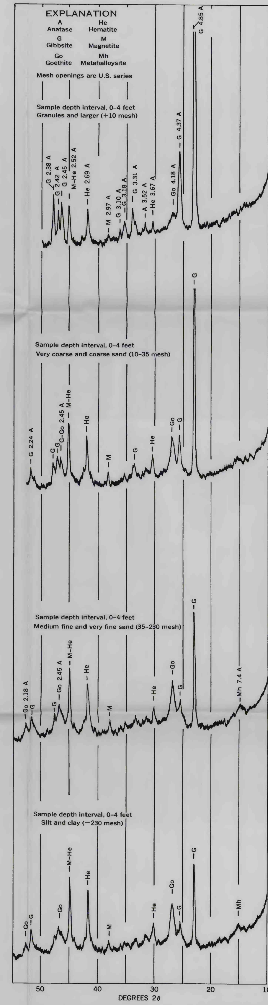
E.—SIEVED FRACTIONS FROM FERRUGINOUS BAUXITE AND SAPROLITE AUGER HOLE GF-46 (PL. 3), KAUI. FeK \alpha_1 FILTERED RADIATION
