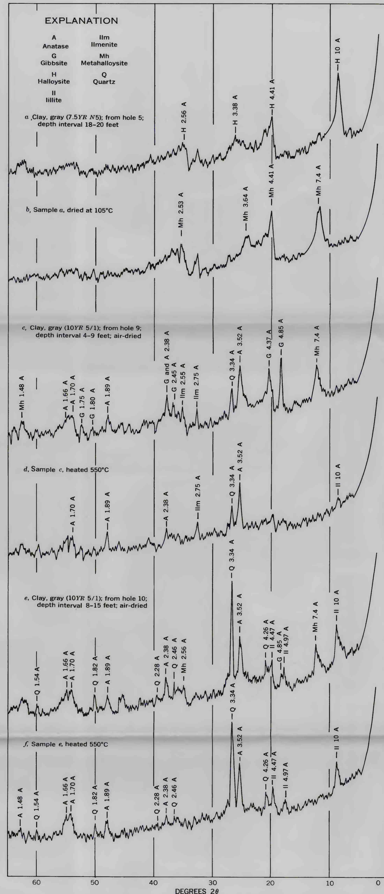
D.—PLASTIC CLAY FROM ALAKAI SWAMP, KAUI (PL. 5). CuK \alpha_1 FILTERED RADIATION
