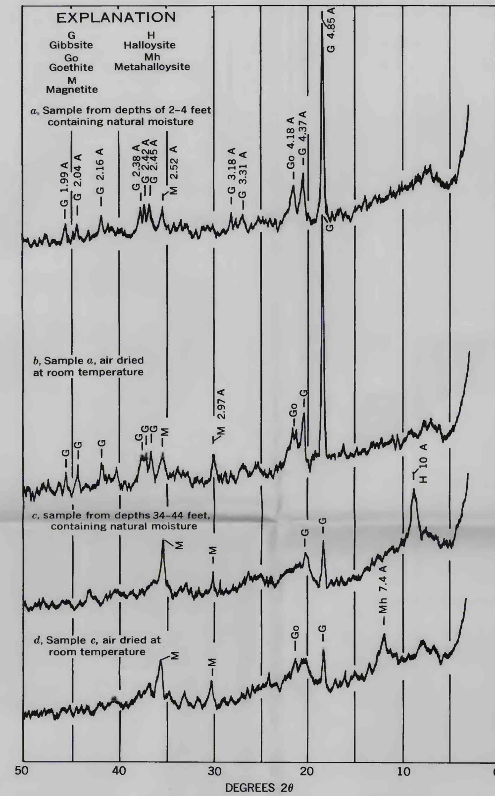
B.—WHOLE SAMPLES OF FERRUGINOUS BAUXITE AND SAPROLITE, AUGER HOLE KI-56, KAUI (PL. 3). CuK \alpha_1 FILTERED RADIATION
