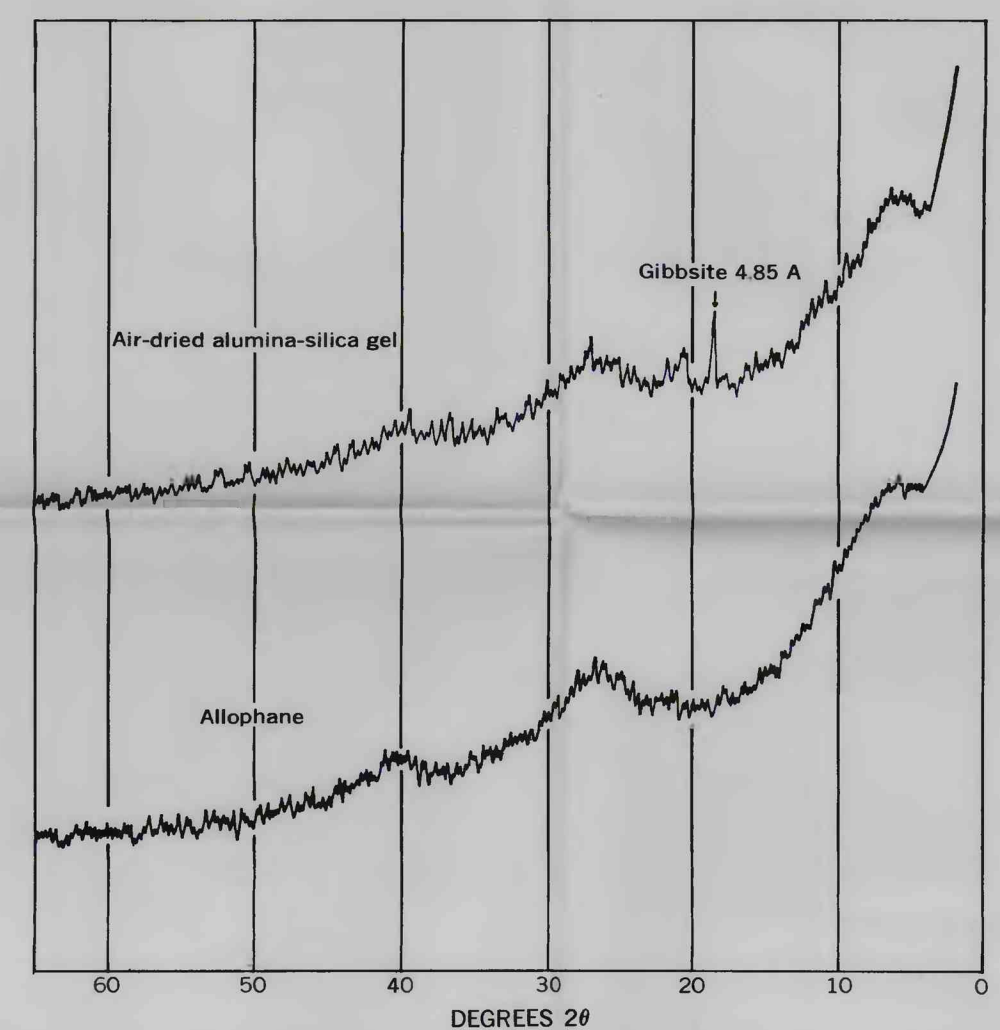
C.—ALUMINA-SILICA GEL AND ALLOPHANE, MAUI. CuK \alpha_1 FILTERED RADIATION
