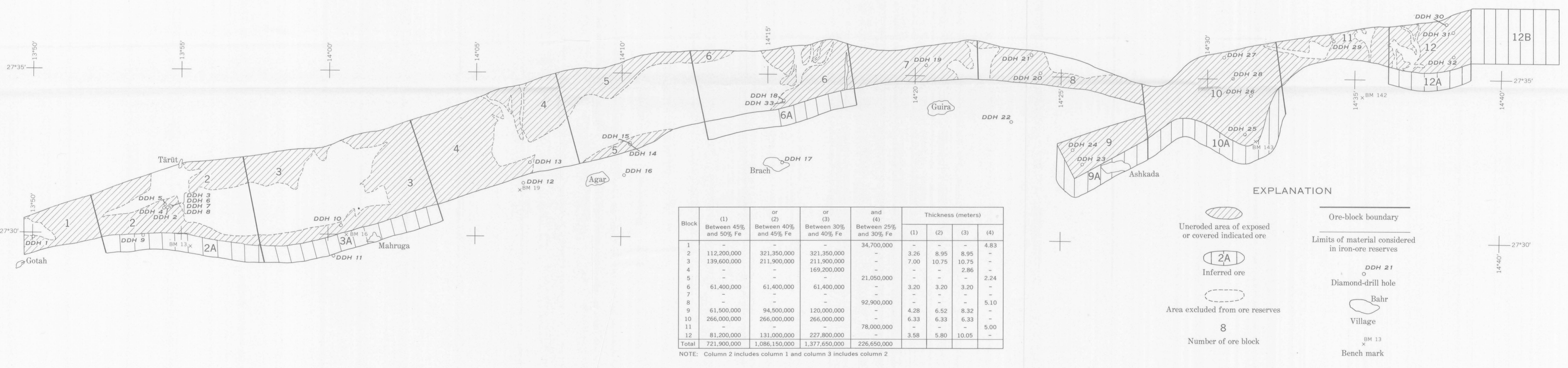
LIMITS OF INDICATED AND INFERRED ORE AND ORE BLOCKS
