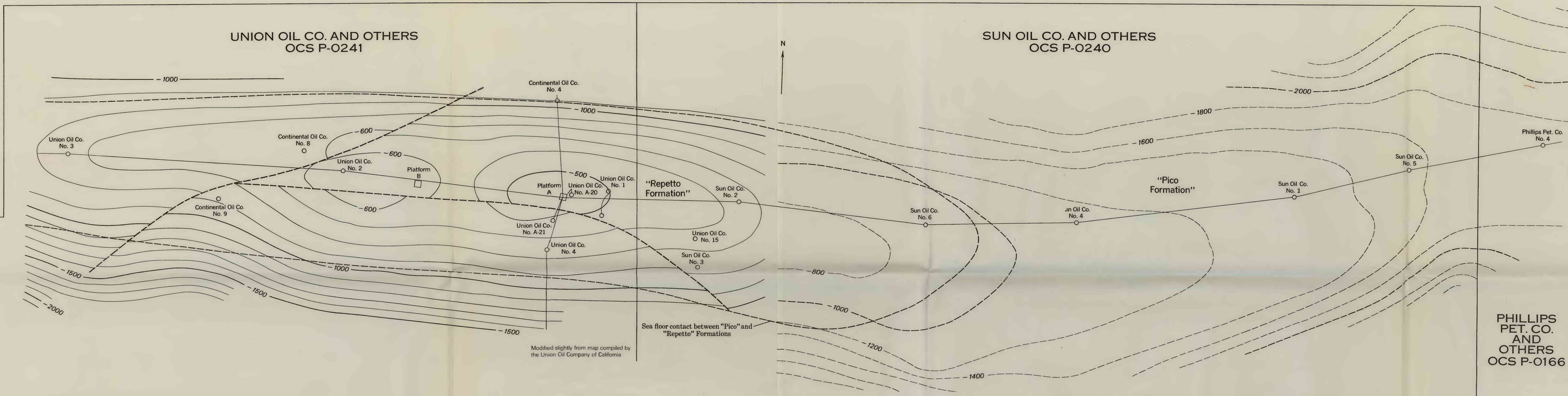
MAP SHOWING STRUCTURE CONTOURS BASED ON WELL LOGS AND SEISMIC-REFLECTION DATA
