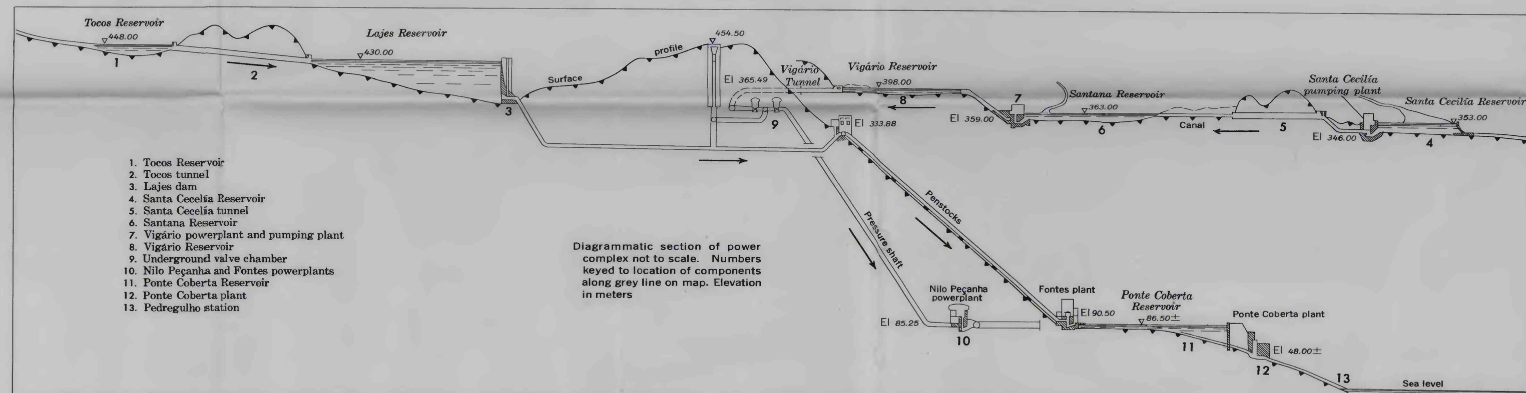
MAP AND DIAGRAMMATIC SECTION SHOWING HYDROELECTRIC COMPLEX AND MAIN WATER-SUPPLY SYSTEM OF THE CITY OF RIO DE JANEIRO, BRAZIL
