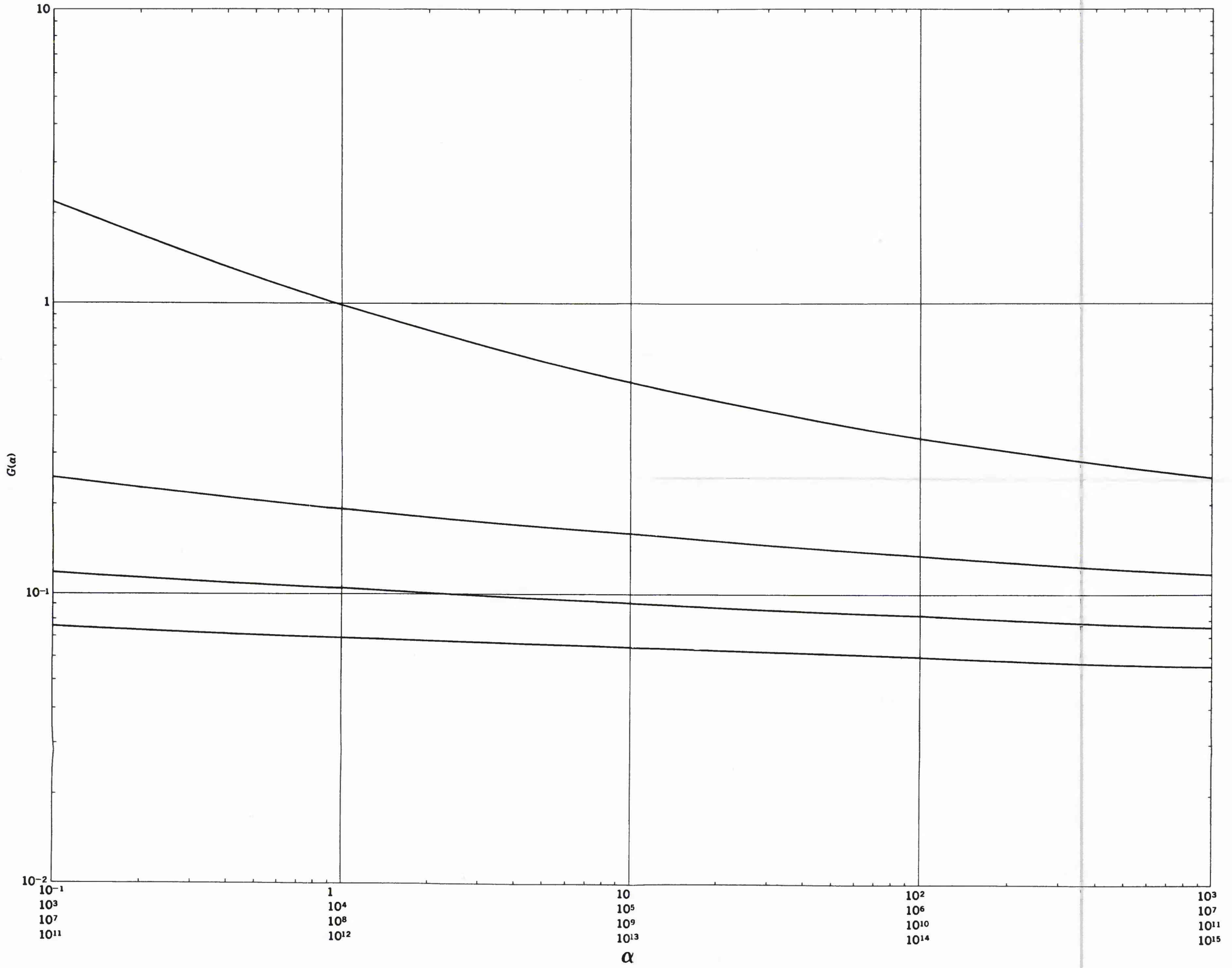
LOGARITHMIC PLOT OF \alpha VERSUS G(\alpha)
