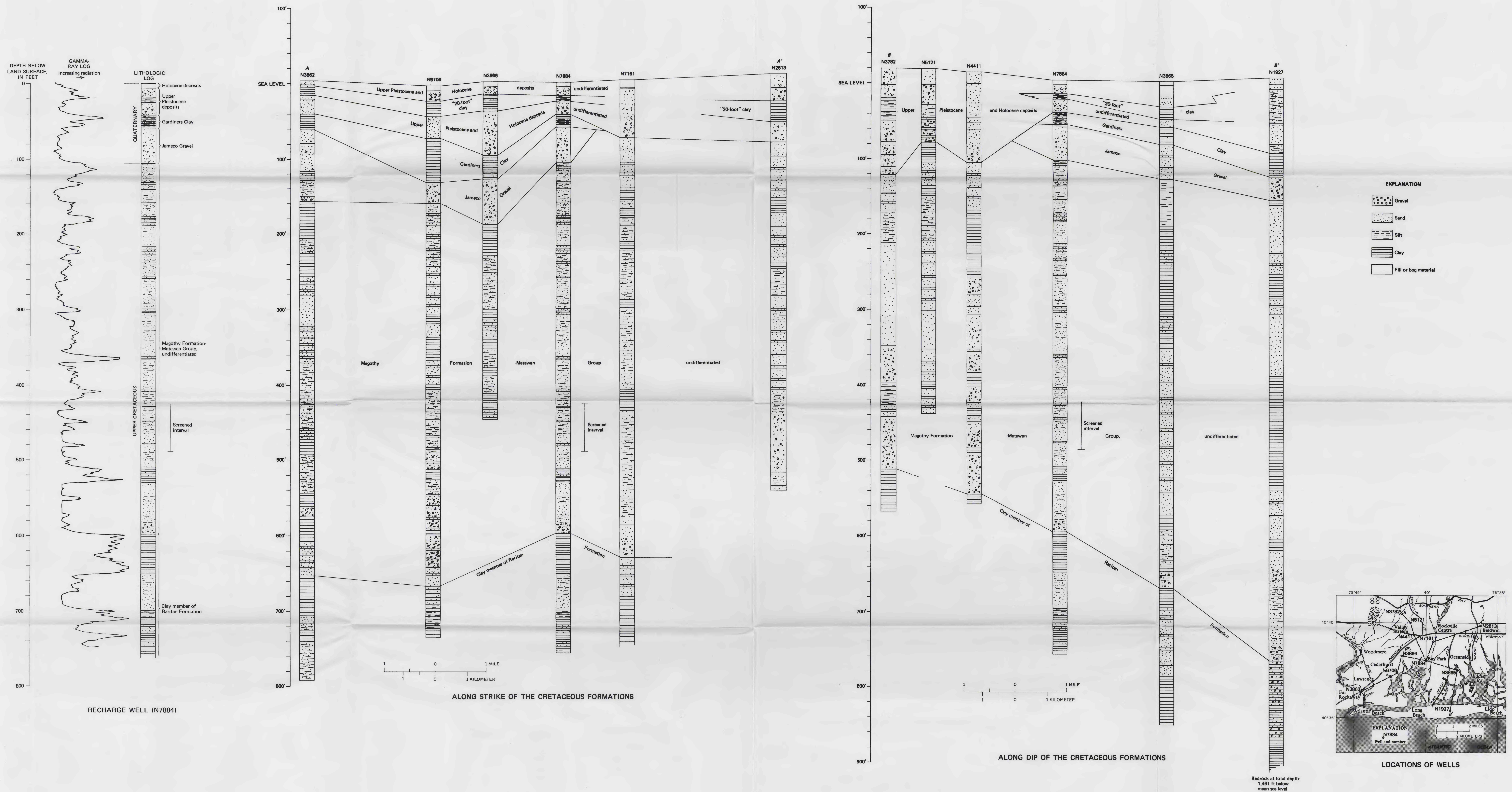
LITHOLOGIC SECTIONS THROUGH THE BAY PARK SITE AND ADJACENT AREA, LONG ISLAND, NEW YORK
