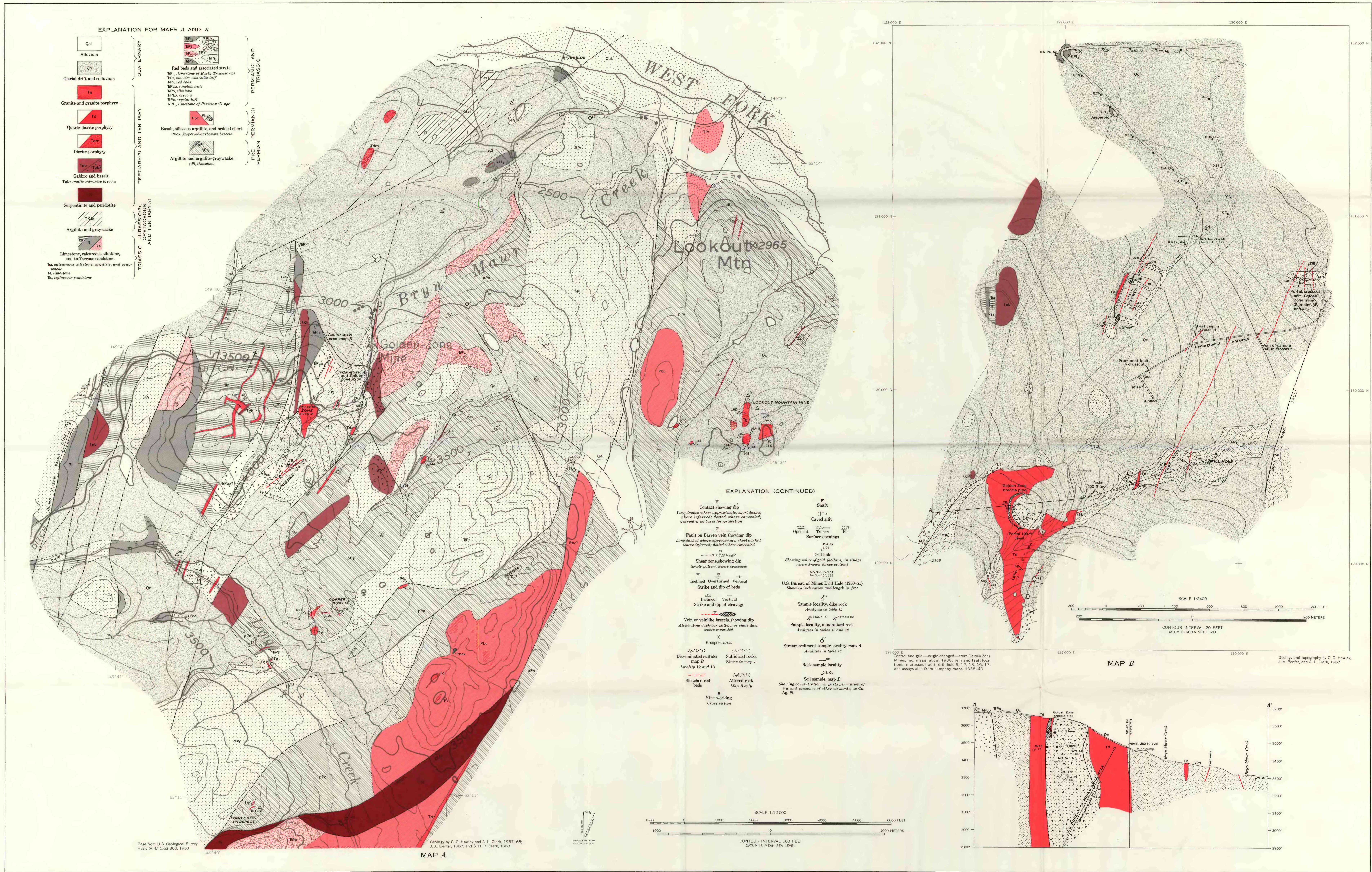
GEOLOGIC MAPS AND SECTION NEAR THE GOLDEN ZONE MINE, UPPER CHULITNA DISTRICT, ALASKA
