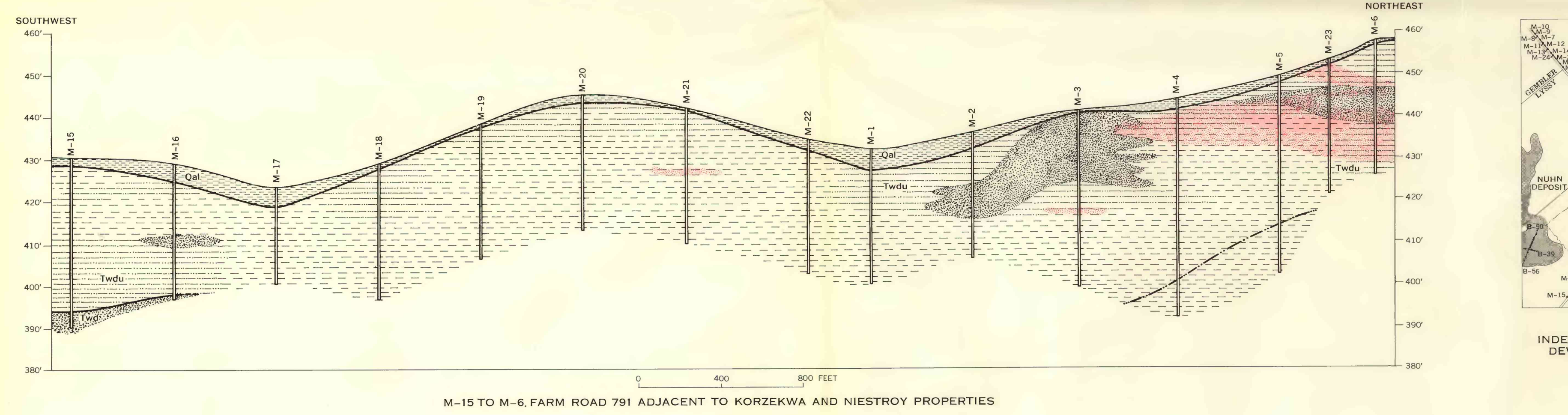
SECTIONS AND FENCE DIAGRAM SHOWING LITHOLOGY AND DISTRIBUTION OF URANIUM, TORDILLA HILL-DEWEESVILLE AREA, KARNES COUNTY, TEXAS
