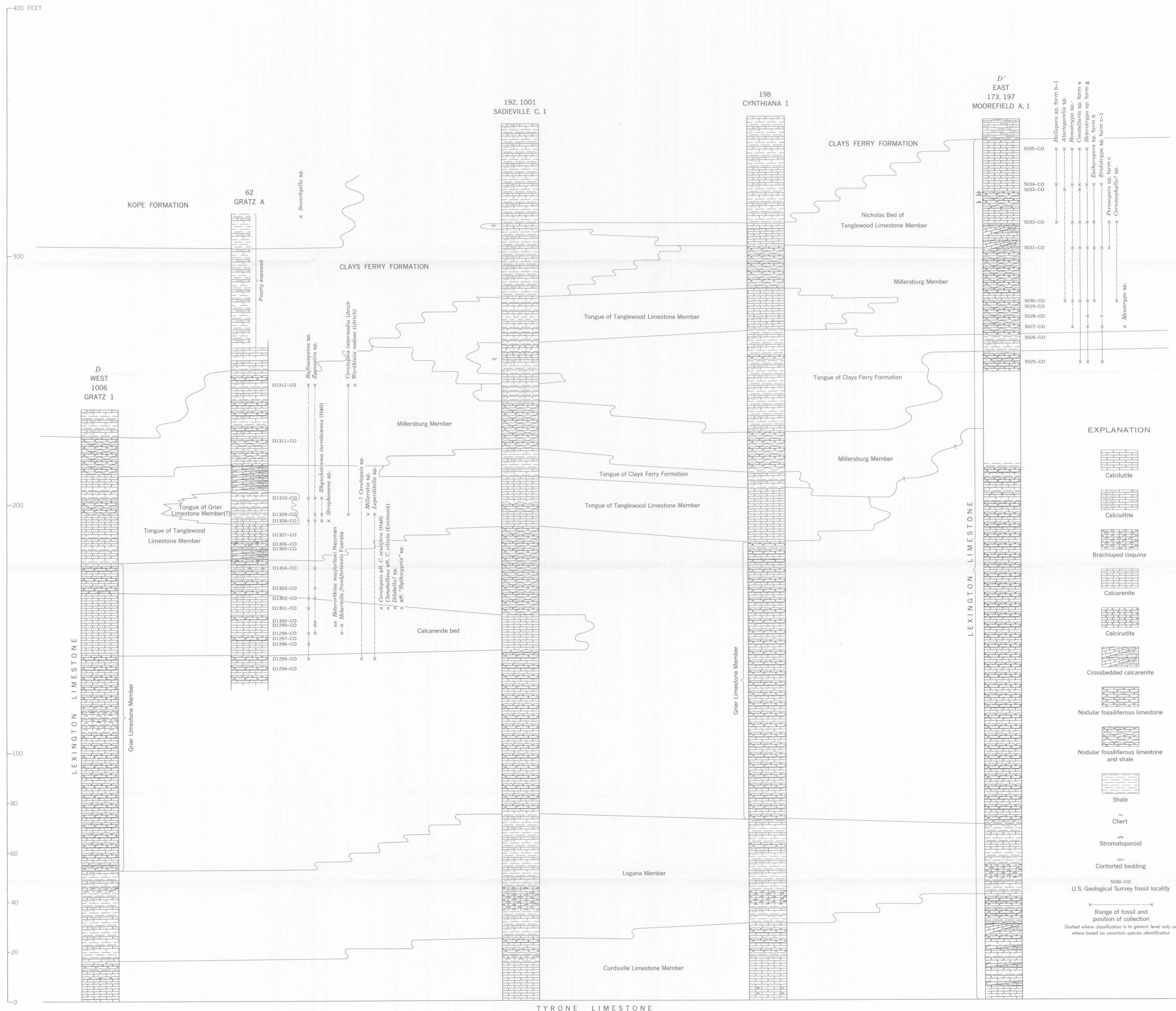
STRATIGRAPHIC SECTIONS OF THE LEXINGTON LIMESTONE, CENTRAL KENTUCKY, SHOWING RANGES OF FOSSILS ALONG LINE D-D'
