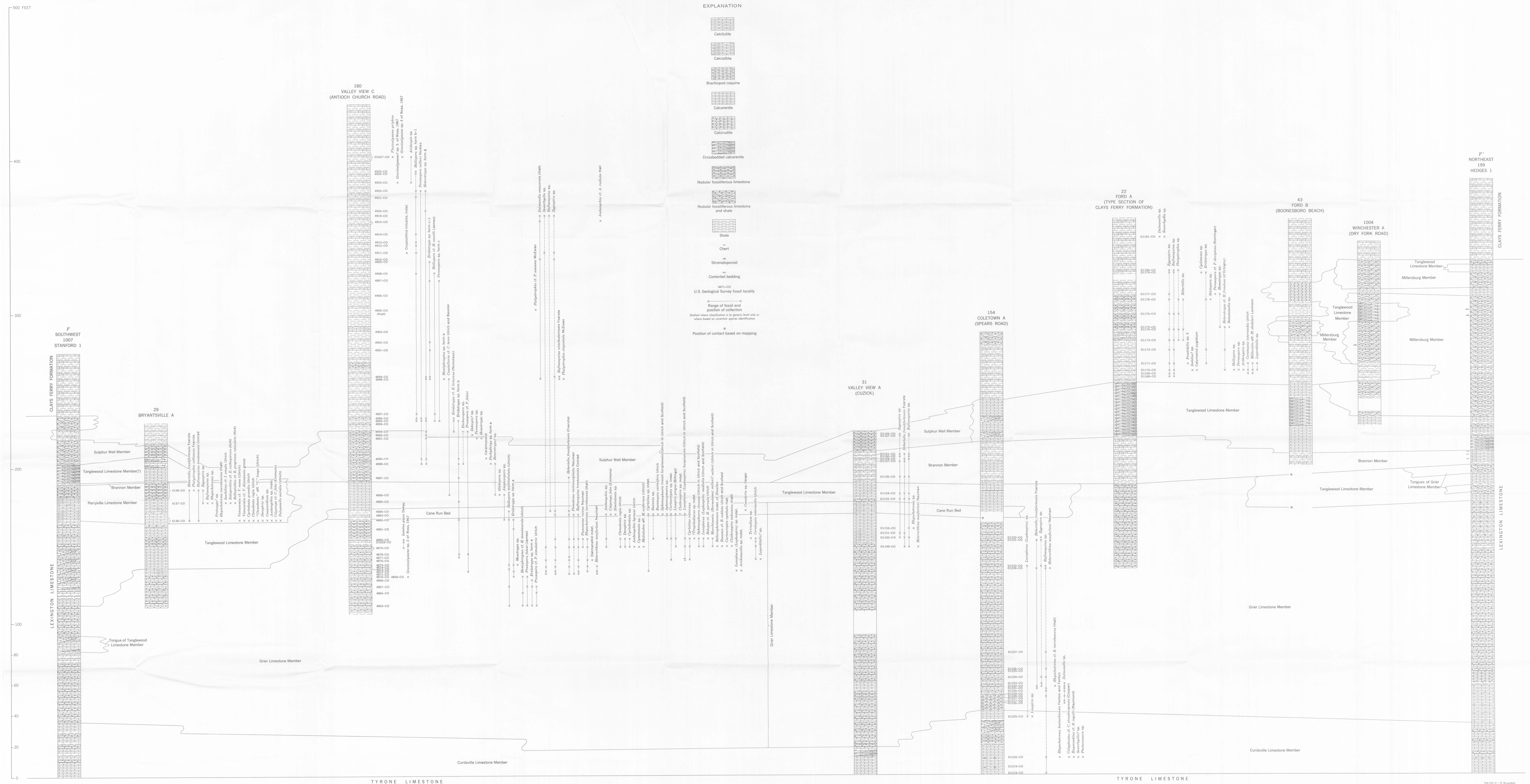
STRATIGRAPHIC SECTIONS OF THE LEXINGTON LIMESTONE, CENTRAL KENTUCKY, SHOWING RANGES OF FOSSILS ALONG LINE F-F'
