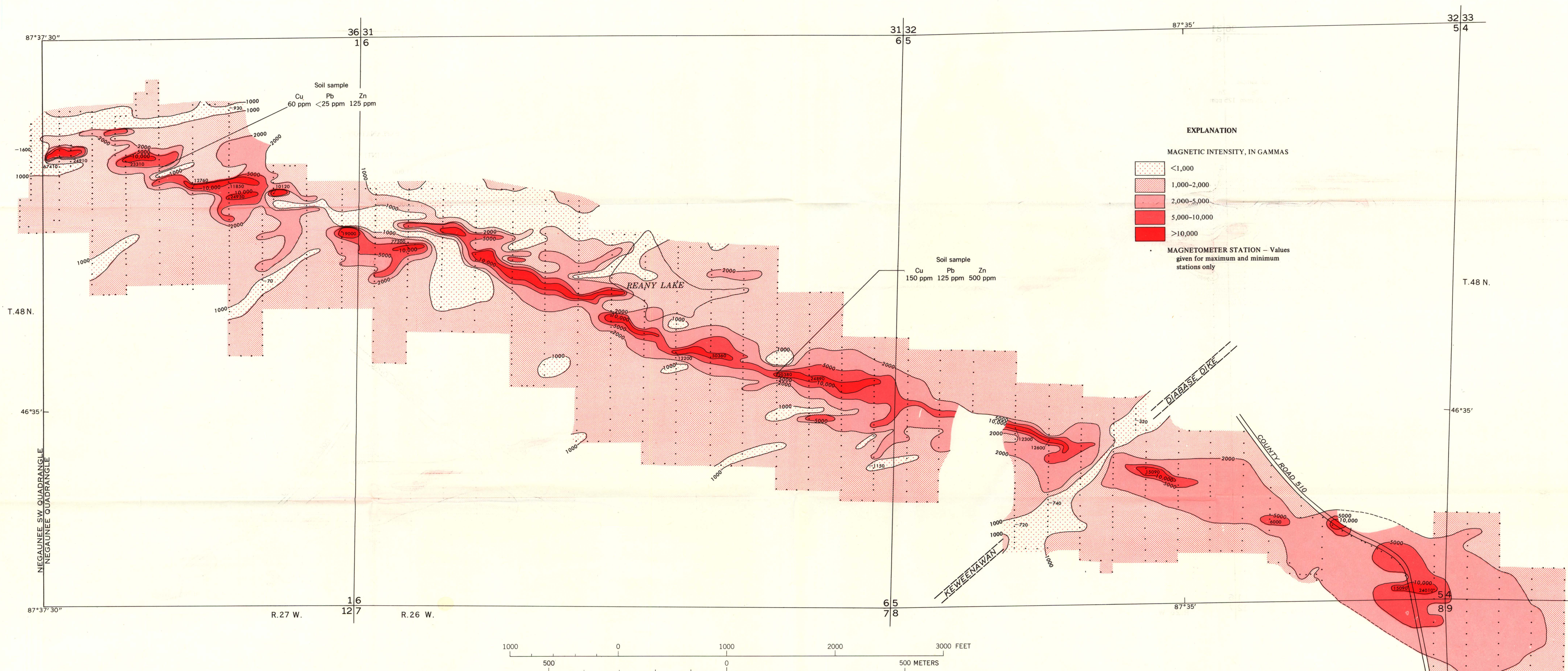
GROUND-MAGNETIC MAP OF PART OF AREA NORTH OF DEAD RIVER BASIN, NEGAUNEE QUADRANGLE, MARQUETTE COUNTY, MICHIGAN
