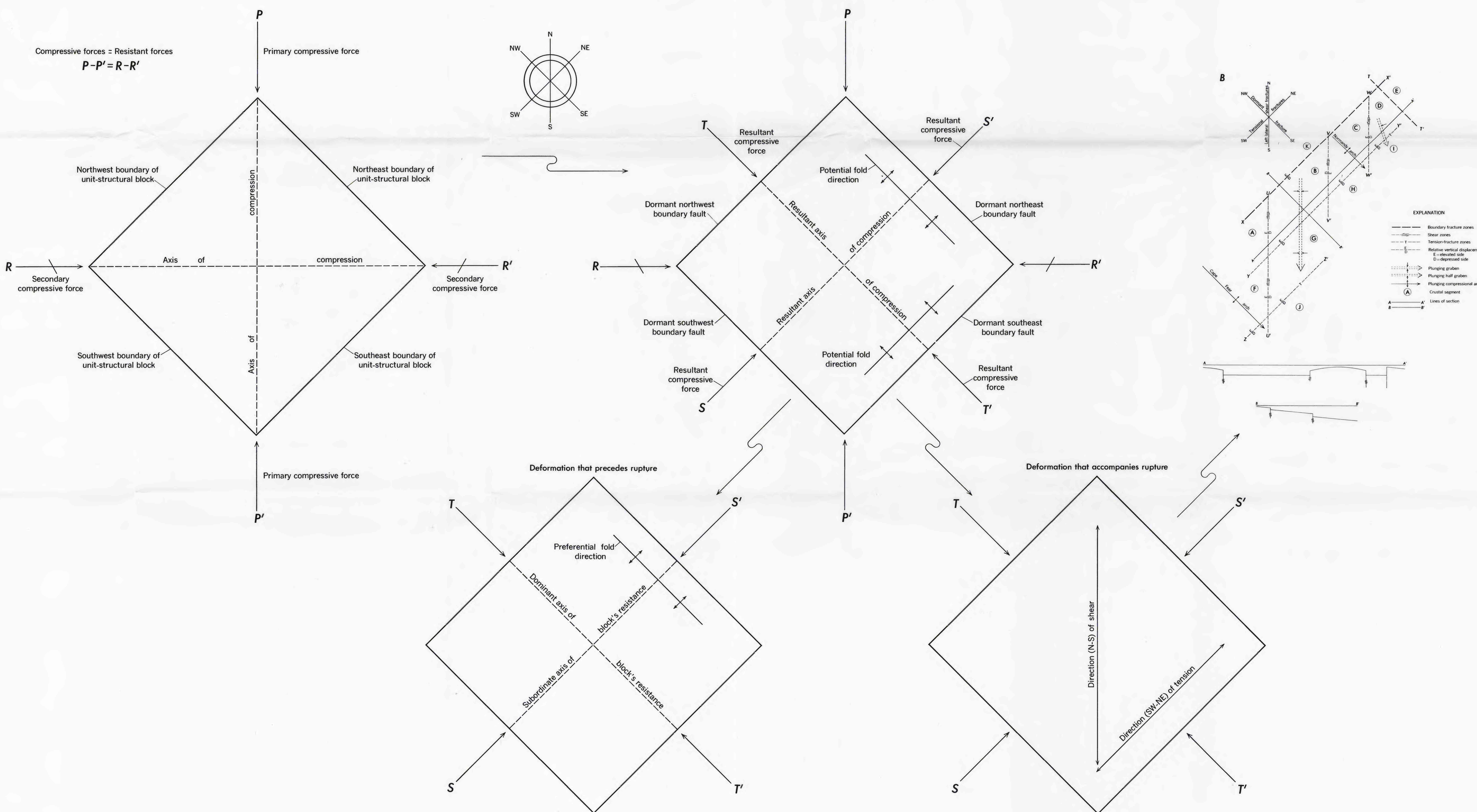
B. DEFORMATION (PHASE 2 AND PHASE 3) DURING A SECOND-ORDER TECTONIC STAGE
