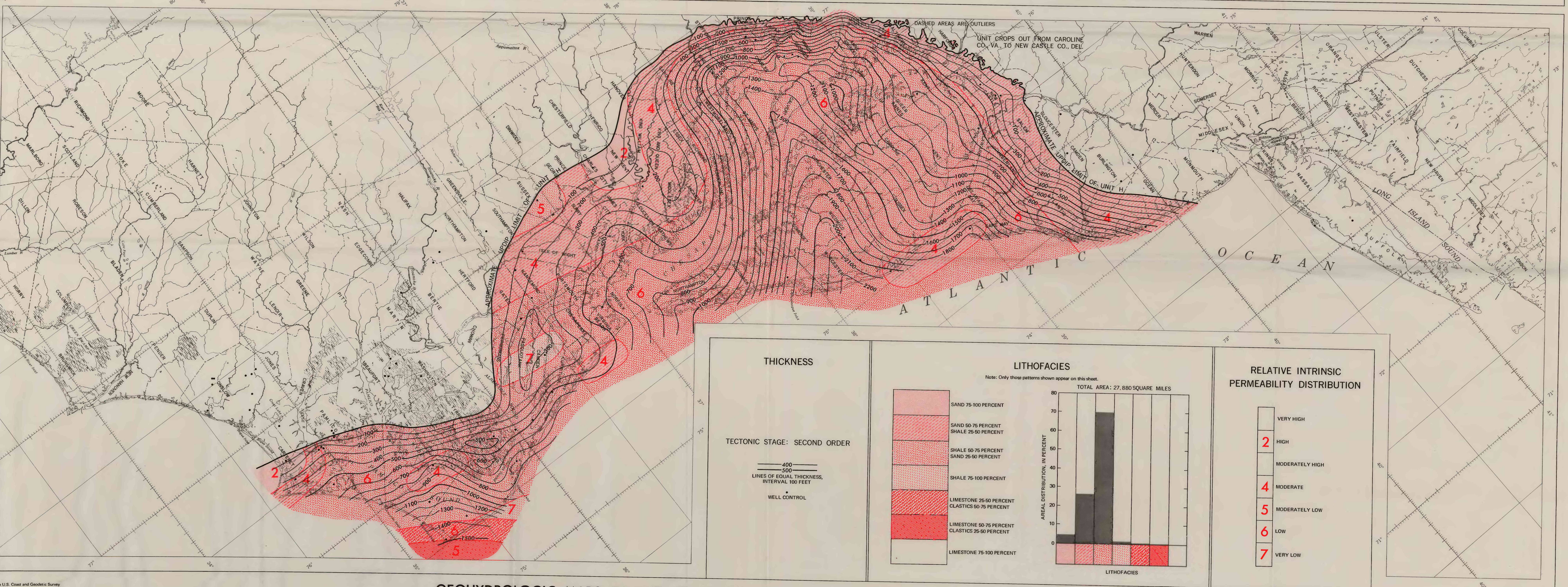
GEOHYDROLOGIC MAPS OF THE ATLANTIC COASTAL PLAIN, NORTH CAROLINA TO NEW YORK, CRETACEOUS AND LATE JURASSIC(?)—UNIT H
