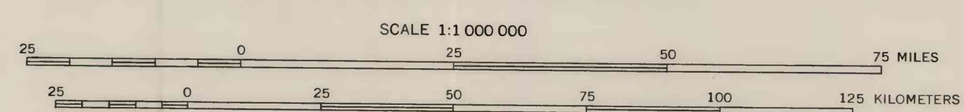
GEOHYDROLOGIC MAPS OF THE ATLANTIC COASTAL PLAIN, NORTH CAROLINA TO NEW YORK, CRETACEOUS—UNIT G
