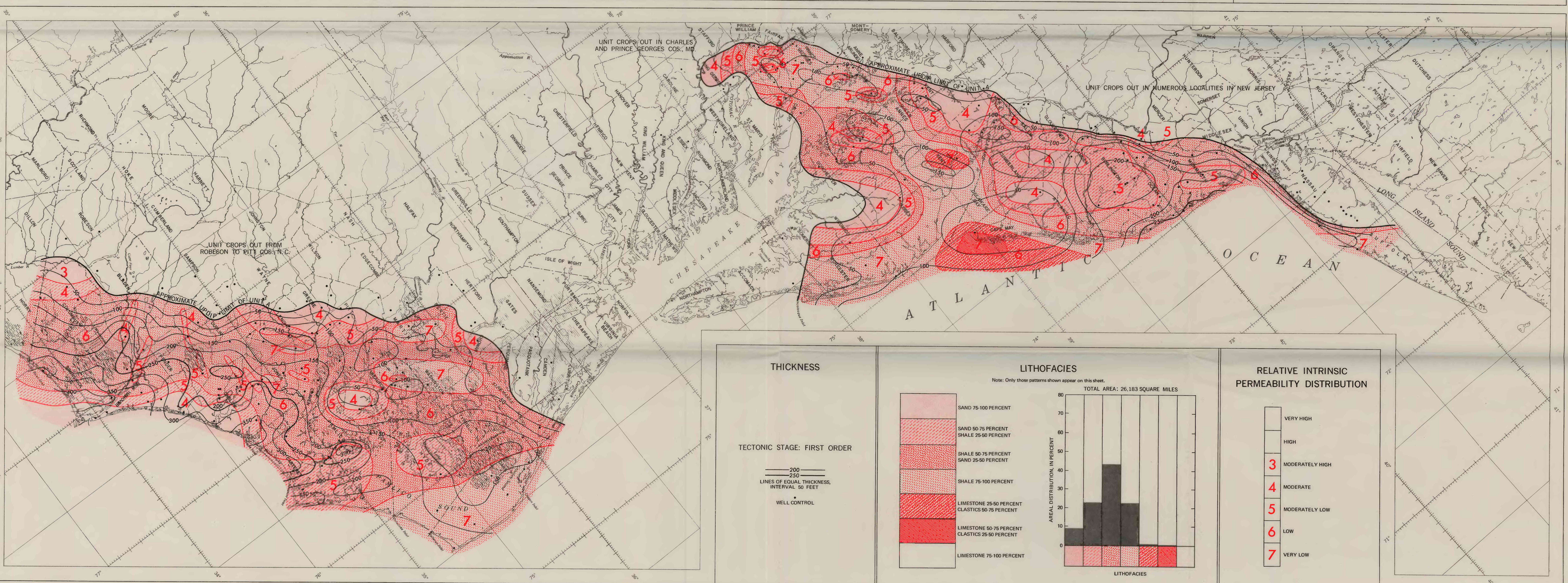
GEOHYDROLOGIC MAPS OF THE ATLANTIC COASTAL PLAIN, NORTH CAROLINA TO NEW YORK, CRETACEOUS—UNIT A
