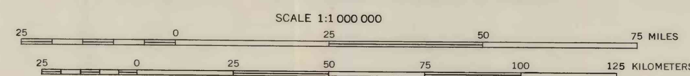
GEOHYDROLOGIC MAPS OF THE ATLANTIC COASTAL PLAIN, NORTH CAROLINA TO NEW YORK, ROCKS OF MIDWAY AGE
