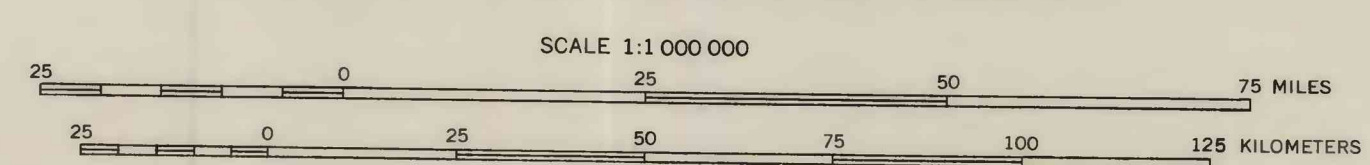
GEOHYDROLOGIC MAPS OF THE ATLANTIC COASTAL PLAIN, NORTH CAROLINA TO NEW YORK, ROCKS OF SABINE AGE
