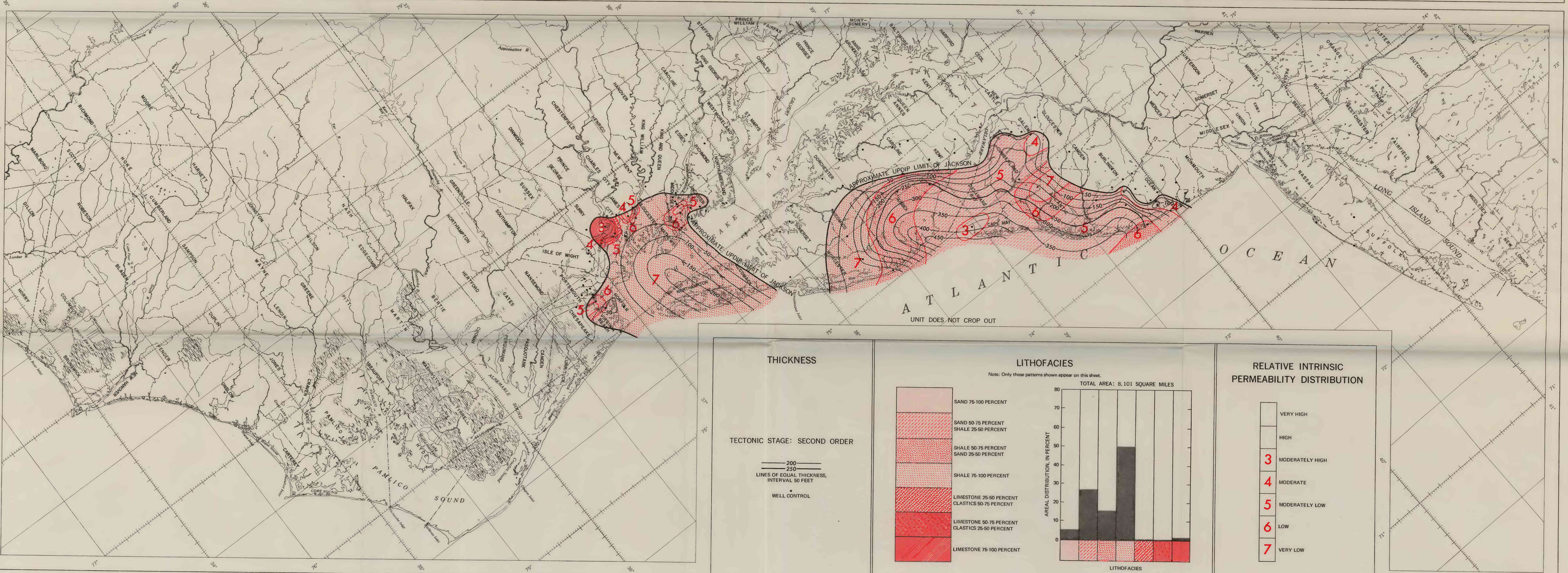
GEOHYDROLOGIC MAPS OF THE ATLANTIC COASTAL PLAIN, NORTH CAROLINA TO NEW YORK, ROCKS OF JACKSON AGE
