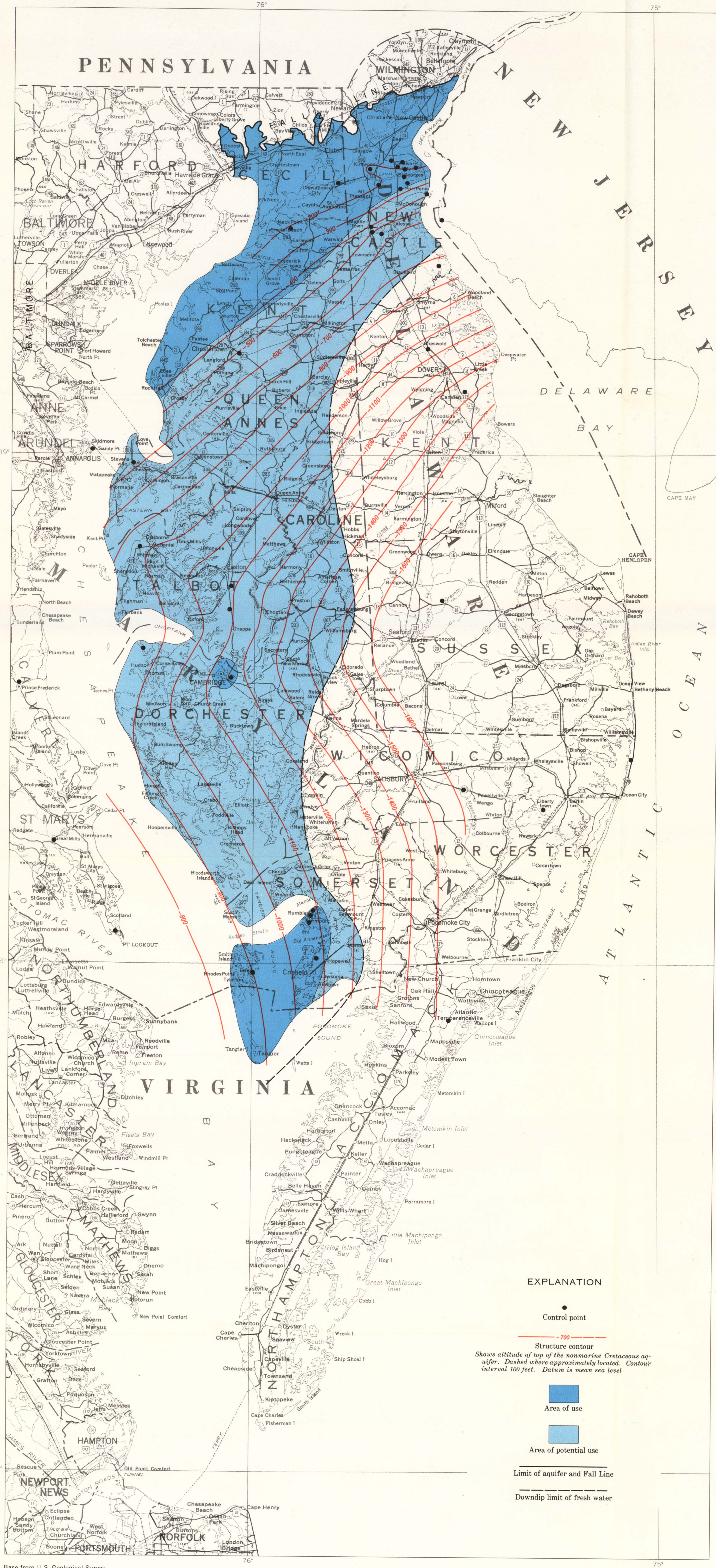
CONFIGURATION OF THE TOP AND AREAS OF USE AND OF POTENTIAL USE OF THE NONMARINE CRETACEOUS AQUIFER
