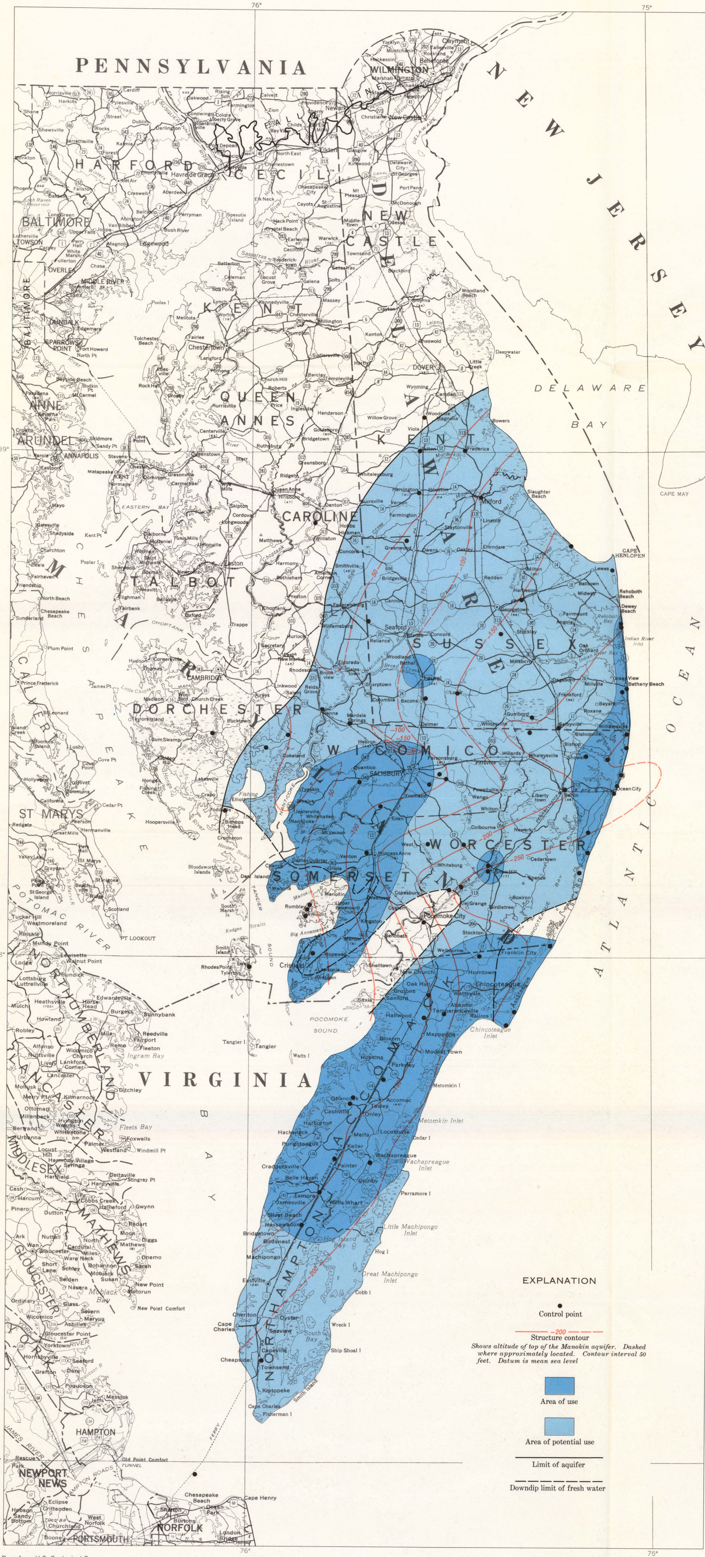
CONFIGURATION OF THE TOP AND AREAS OF USE AND OF POTENTIAL USE OF THE MANOKIN AQUIFER
